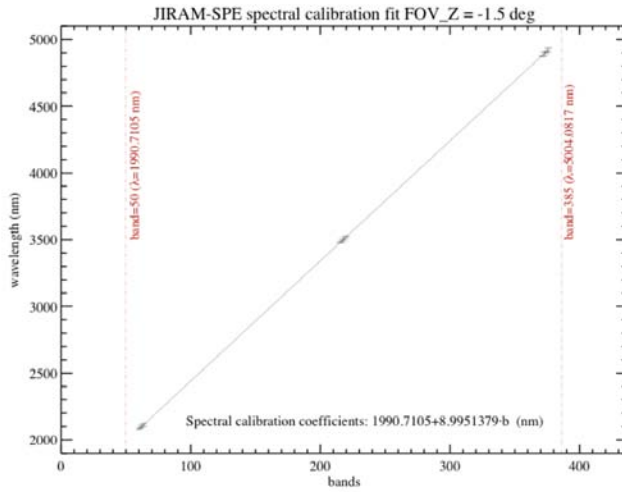
Fig. 15 Spectral calibration parameters retrieved for JIRAM-SPE negative extreme samples ( FOVz = -1.5 \text{ deg} ). The crosses correspond to the monochromator’s spectral scans (centers and FWHMs) taken around 2100, 3500, 4900 nm . The best-fit line and parameters ( \lambda_0 , SSI) are indicated. The two vertical lines correspond to the spectral range extremes.
