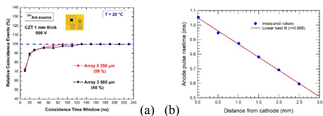
Figure 11: (a) Relative coincidence events (%) of the central pixel, for the 500 \mu\text{m} array 3 (black points) and 250 \mu\text{m} array (red points), with the adjacent pixels at different CTWs. The percentage values of the coincidence events of central pixel with all pixels, for both arrays, are also shown (CTW of 200 ns); (b) the measured strong dependence of the anode pulse rise time from the photon interaction position across the cathode-anode direction.
