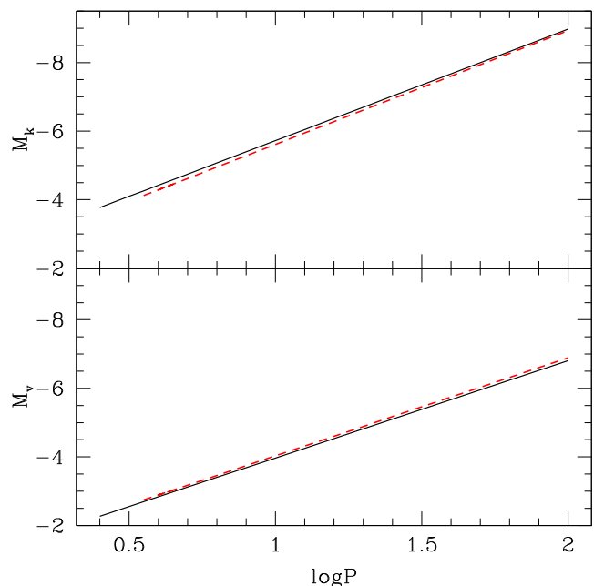
Figure 4. Comparison between the V (bottom panel) and K (top panel) relations with Y = 0.25 (black solid line), Y = 0.35 (red dashed line).
