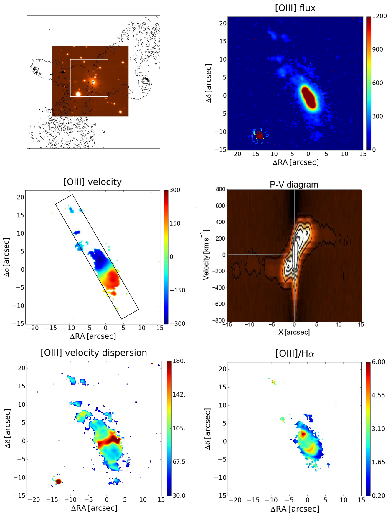
Fig. B.4. 3C 403, FR II/HEG, 1'' = 1.15 kpc. Top left: radio contours overlaid onto the Muse optical continuum image. Top right: [O III] emission line image extracted from the white square in the top left panel. Middle: velocity field from the [O III] line and PV diagram (the synthetic slit is centered on the nucleus, has a width of 30 pixels and it is oriented at an angle of -60^\circ from the X axis). Bottom: [O III] velocity dispersion and [O III]/H \alpha ratio.
