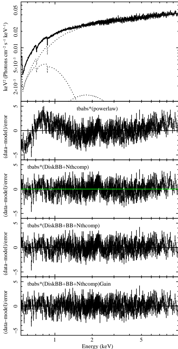
Figure 9. (Top panel) XMM-Newton EPIC-pn hard state spectrum fitted by the best fit model (disc black body plus blackbody and a dominant Comptonisation components absorbed by neutral material). No signs of ionised absorption is present. (Centre top panel) Residuals once the data are fitted with an absorbed power law. (Centre panel) Residuals after fitting with an absorbed disk black body plus Comptonisation model. (Centre bottom panel) Residuals after the addition of a black body component. (Bottom panel) Residuals after the consideration of a gain offset in the response files.
