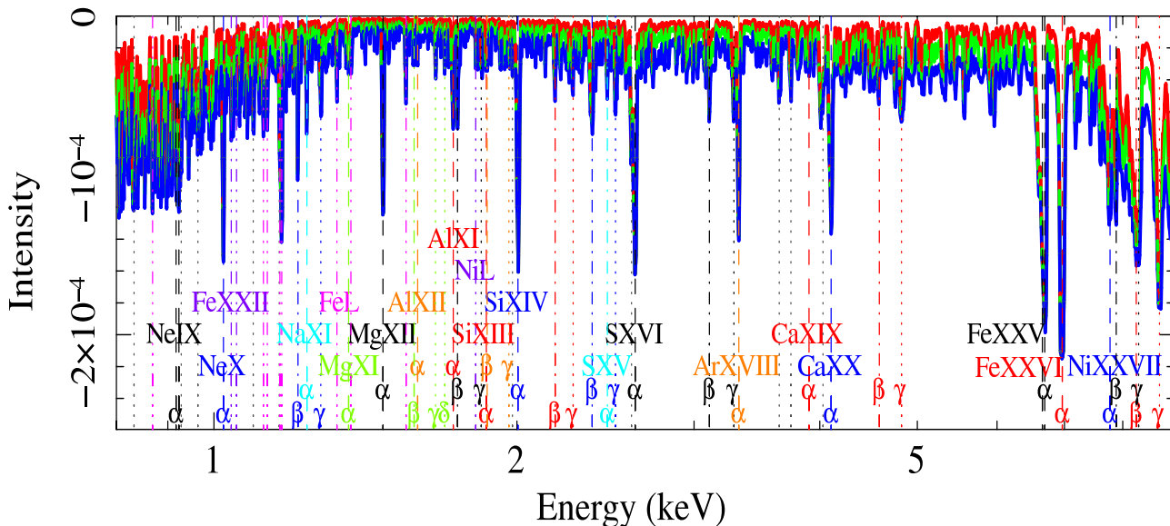
Figure 4. Residuals to the presence of narrow ( \sigma = 1 eV) absorption lines in the Chandra HETG (HEG+MEG) spectra. The red, green and blue solid lines show the 68, 90 and 99 % confidence contours. Sixty absorption lines are detected. We highlight with a vertical line each detected absorption feature. The same colour is used for features associated to the same series. In particular, the energies of the \alpha , \beta and \gamma transitions are reported with dashed, dash-dotted and dotted lines, respectively. Absorption lines associated with Fe L features are highlighted with magenta dot-dot-dot-dashed lines (in violet is the density sensitive Fe XXII doublet). Unidentified lines are shown with grey dotted lines.
