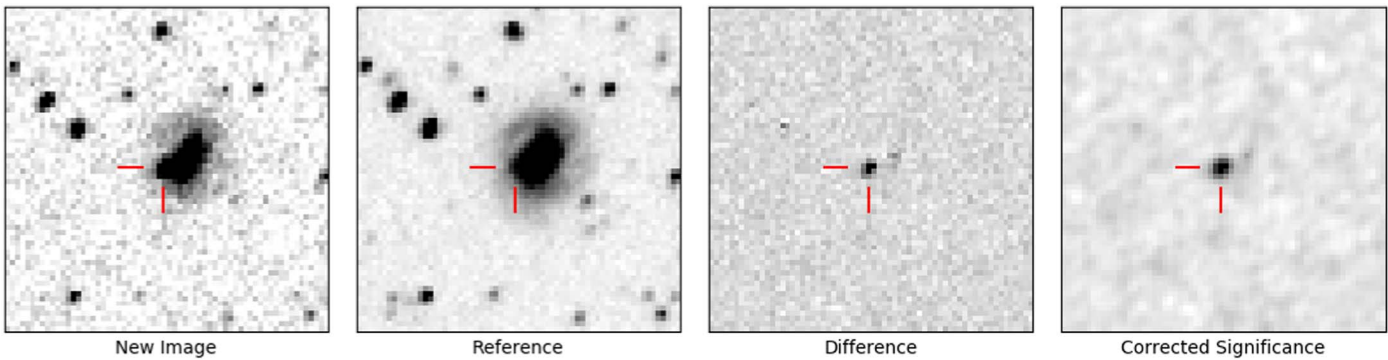
Figure 5. CSS imaging of AT 2019bfn, a known transient found within the data for the S190425z event. Left: the new image created from the median of the four CSS images with a mid-time of 2019 April 25 09:35:48.12 UTC and \delta t \approx 1.29 hr after the GW event. Second: the reference image from the deep templates created with 62 30 s images, giving a total exposure time of 31 minutes. Third: the difference image produced by the image subtraction. Right: corrected significance (Scorr) image showing the significance of the detection in the difference image. AT 2019bfn was detected with an S/N of 15.
