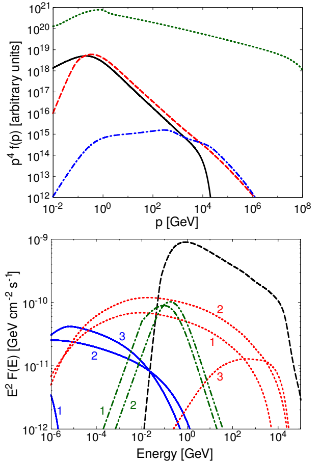
Figure 3. Particle and photon spectra in Model B. The line style is the same as in Figure 2.
