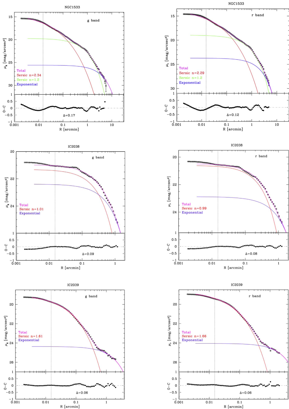
Figure 14. Azimuthally averaged (and PSF deconvolved for NGC 1533) surface brightness profiles in the g band (left panels) and in r band (right panels) and the residuals between the observed surface brightness and the best fit; the gray dashed line indicates the zero level. Top panels refer to NGC 1533, middle panels to IC 2038, and bottom panels to IC 2039. Red and green solid lines represent Sérsic laws, blue solid line represent exponential function, and the magenta solid line is the resulting best-fit interpolation. The vertical dotted line delimits the regions affected by seeing, which are excluded from the fit.
