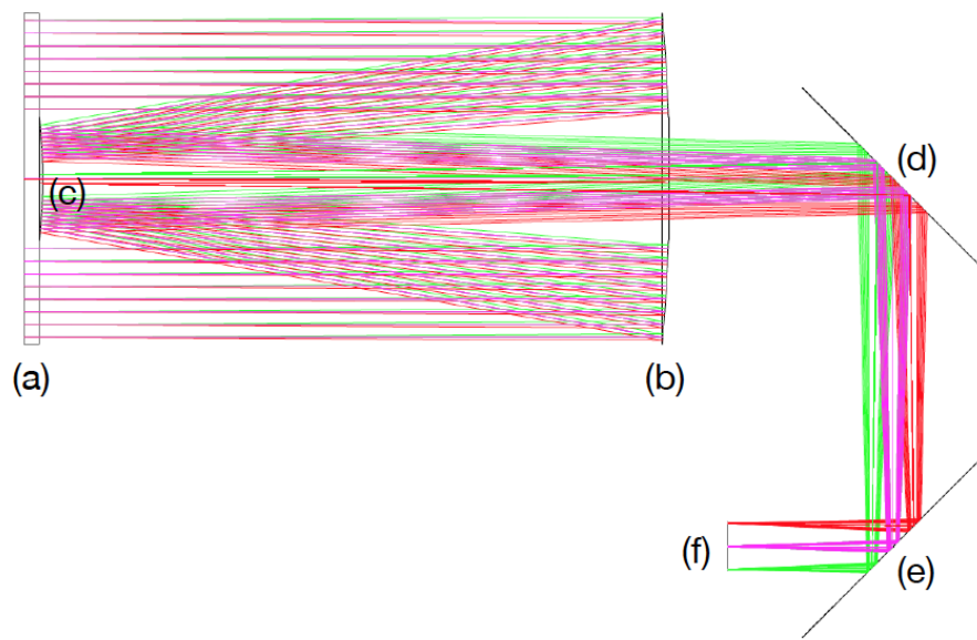
Figure 3: SPEC optical design. In order: corrective Schmidt lens (a); primary spherical mirror (b); secondary aspherical mirror (c); first fold mirror (d); second fold mirror (e); camera sensor (f). The three different colours represent the 5 different analysed FoVs: green, purple, yellow and red rays represent the (0, -0.3) , (0.3, 0) , (-0.3, 0) and (0, 0.3) fields respectively; while the blue rays represent the optical axis aligned field (0, 0) .
