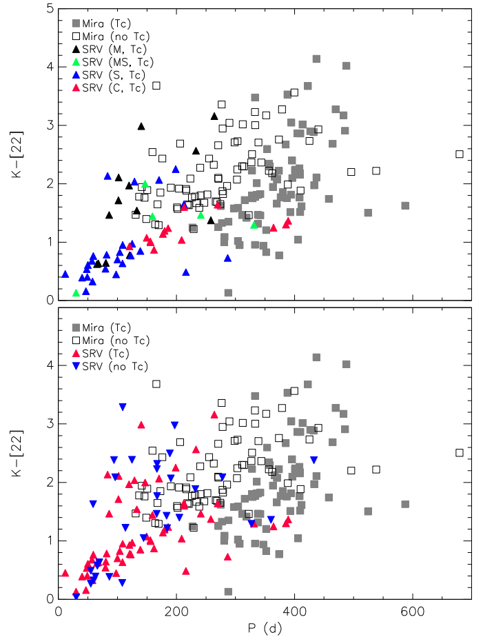
Fig. 6. Upper panel: P vs. K - [22] diagram including Tc-rich SRVs (triangles). Different spectral types are colour-coded, see legend. Lower panel: same as upper panel, but showing M-type Tc-poor (downward-pointing blue triangles) and Tc-rich (upward-pointing red triangles) SRVs. Mira stars are shown in both panels as open and filled grey squares.
