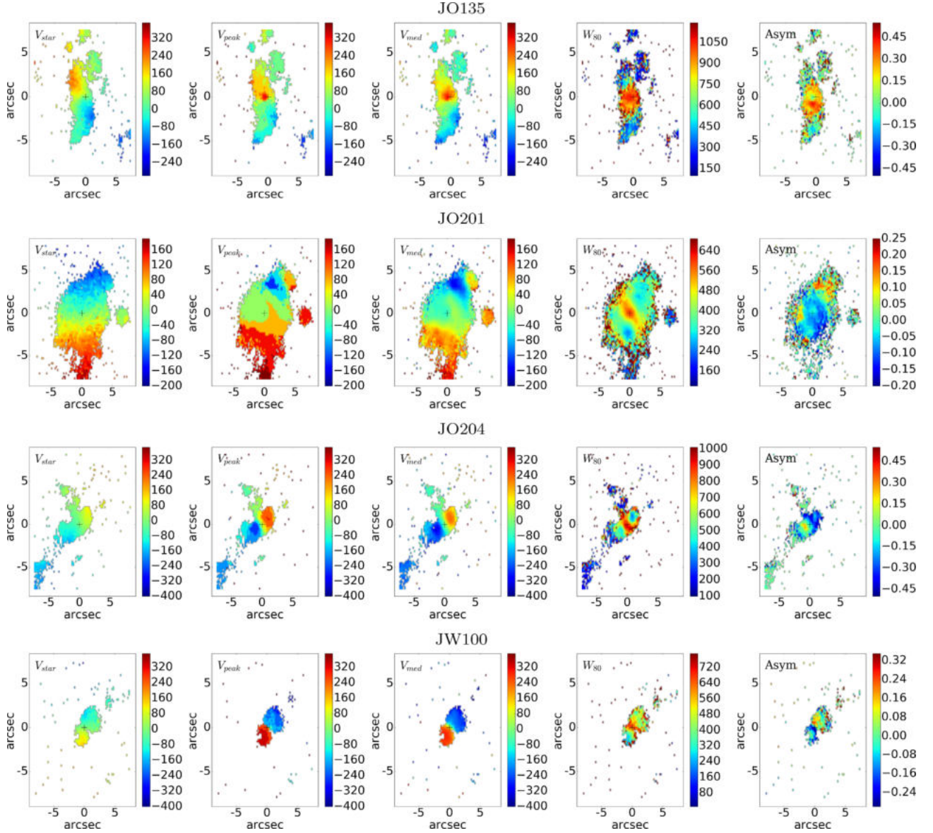
Figure 8. For each galaxy hosting an AGN, the plots display the spatial distribution of the stellar velocity ( \text{km s}^{-1} ) (first panel) and of the following parameters (see text for details) derived from the [O III] line: peak and median velocity ( \text{km s}^{-1} ); W_{80} ( \text{km s}^{-1} ); asymmetry (right-hand panel). In each plot, North is up and East is at left.
