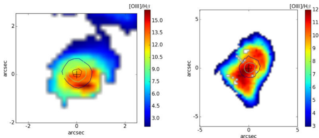
Figure 6. The contour maps showing emission at SN of \sim 5\text{--}20 in the [\text{Fe VII}] \lambda 6087 line are overplotted on the [\text{O III}] \lambda 5007/\text{H}\beta map for the nuclear AGN regions of JO135 ( left ) and JO201 ( right ). The cross displays the position of the peak in [\text{O III}] \lambda 5007 .
