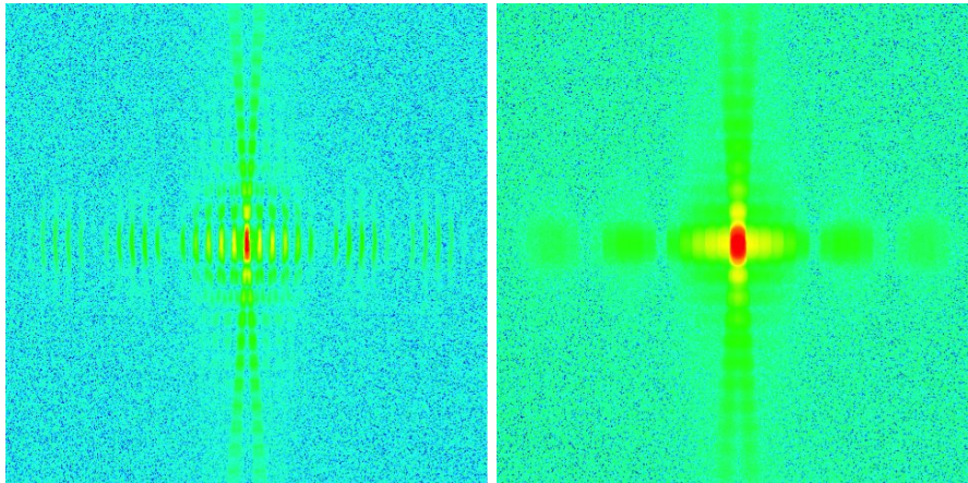
Figure 7. Best-focus configuration of two separated MMs, supposed to have perfect Wolter I surfaces. The simulated detector field is 2 mm and the pixel size is 2 \mu\text{m} . Left: PSF of two MMs illuminated by a 0.25 arcsec source. Right: PSF of two MMs illuminated by a 1 arcsec dimension source.
