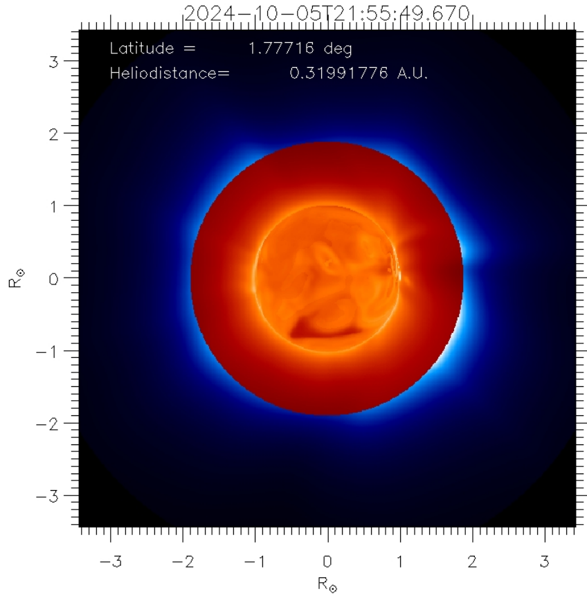
Figure 3. An example of a synthetic image produced by FORWARD: the inner region represent the EUV disk as it will be seen by EUi at 174 Å and the external part is the WL corona.
