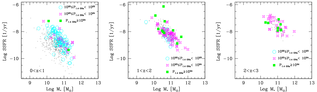
Figure 9. SSFRs as a function of stellar mass for radio-selected AGNs in three different redshift intervals. Sources are colour coded according to their radio luminosity (expressed in [\text{W Hz}^{-1} \text{sr}^{-1}] units). Black dots indicate the distribution observed for radio-selected star-forming galaxies of all radio luminosities.
