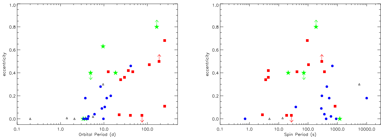
Figure 14. Properties of the sample of HMXBs, in terms of orbital eccentricity versus orbital period ( left panel ) and of eccentricity versus pulsar rotational period ( right panel ). The meaning of the symbols is the same as in Figs. 11 and 12.
