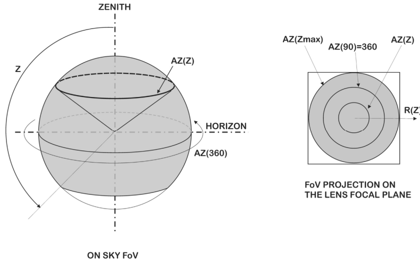
Fig. 5. Azimuth angle as a function of zenith angle.
