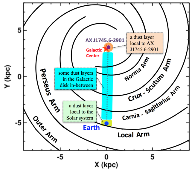
Figure 10. Dust distribution along the LOS of AX J1745.6-2901, as suggested by the best-fit 3-layer and 4-layer models in Table 2, assuming it is in the GC. The schematic of Milky Way’s spiral arms, as shown in Nakanishi & Sofue (2016), Reid et al. (2009), Caswell & Haynes (1987) (also see the review by Bland-Hawthorn & Gerhard (2016)), are also plotted for comparison. Compared to the 2-layer model in Figure 15 of J17, now we identified a third dust layer in the Solar neighbourhood (see Section 6.3), although the second dust layer (cyan region) in the Galactic disk is still poorly resolved.
