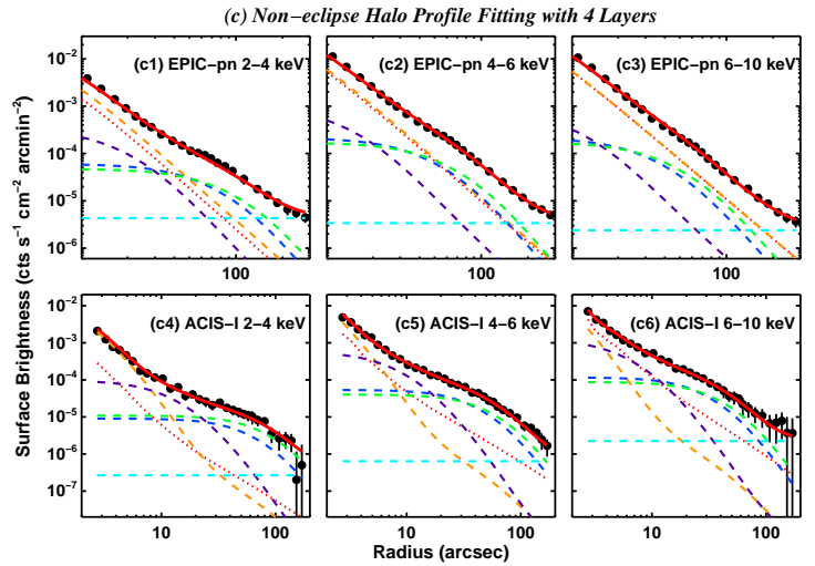
Figure 6. Dust models with 2, 3 and 4 distinct layers along the LOS. In each row, the left-side cartoon shows each layer’s position and parameters. The best-fit results using the COMP-AC-S dust grain model (see Section 5.2.1) are shown on the right side, with dash lines indicating the contribution from every dust scattering component (cyan dash line is the wing component), and the dotted line indicating the instrumental PSF. The results of simultaneous fitting to the eclipse halo profiles using the same model can be found in Fig. A1-A3.
