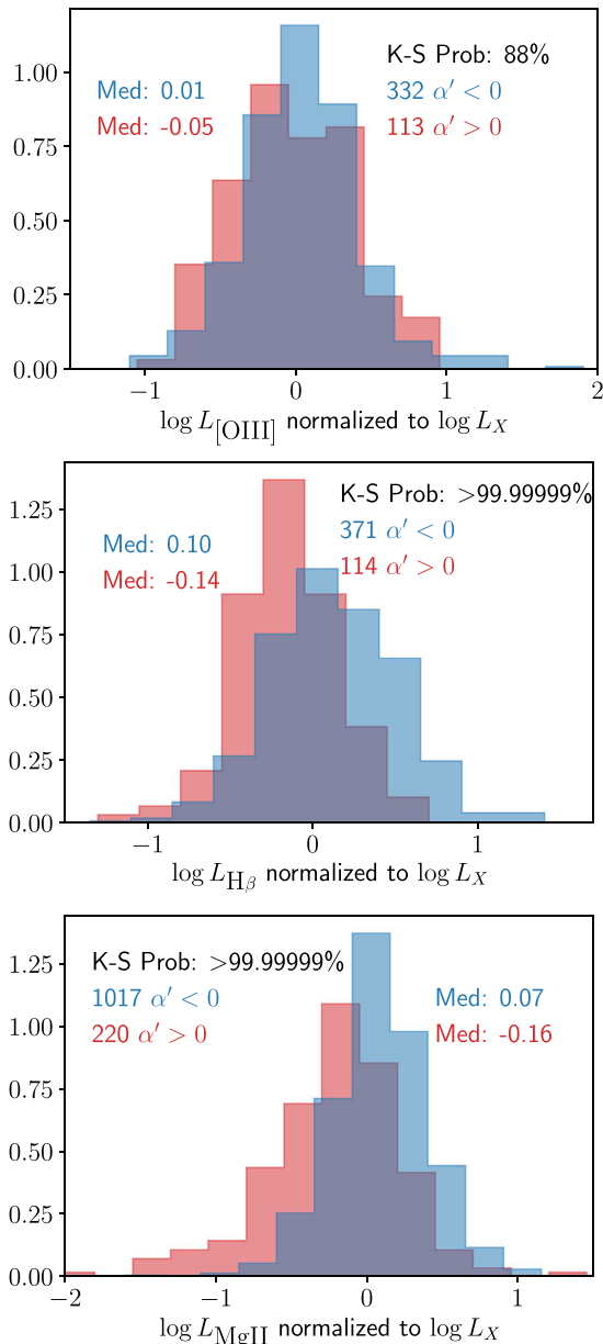
Figure 8. Comparisons of the line luminosities normalized to L_X for [O III], H \beta , and Mg II between the blue ( \alpha' < 0 ) and red ( \alpha' > 0 ) BLAGN using sample ‘1’. We mark the sample sizes, median values, and K–S test probabilities in the figure.
