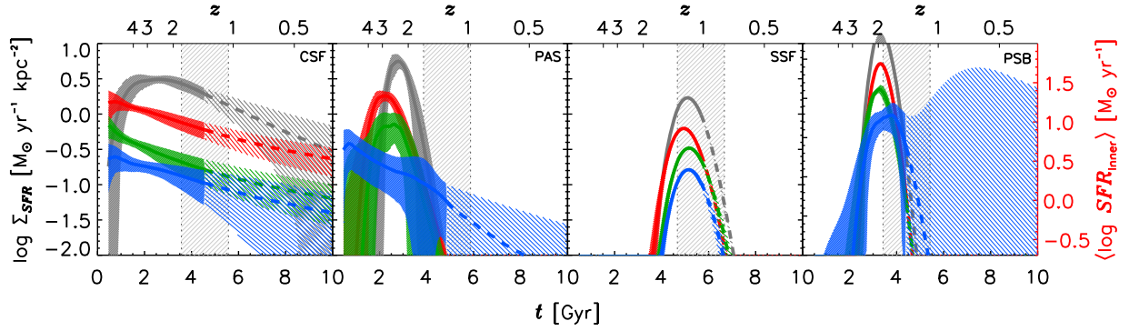
Figure 9. Spatially integrated and resolved SFHs. Colors correspond to previous figures with optimal extraction results (scaled to INNER surface areas) in gray. Epochs before t_{\text{obs}} are shown as solid lines; forecasts are dashes. Vertical bands show the t_{\text{obs}} \pm 1 Gyr interval over which we draw longitudinal inferences (Figure 10). Envelopes show 16th–84th percentile spreads in \text{SFR}(t) from the (T_0, \tau) pyspecfit covariances. All galaxies are observed after their peak, and all but CSF show signs of inside-out/bulge-first growth. INNER SFRs approach/are exceeded by MIDDLE and OUTER SFRs between t_{\text{peak}} and t_{\text{obs}} . Conversely, the relatively diskly CSF (Figure 5) had an \sim constant SFH across its face. SSF is growing strong—proportionately more so at larger r (Figures 3 and 4)—and PAS has been quenching for \sim twice as long as PSB. The right y-axis shows the absolute \text{SFR}_{\text{INNER}} at the sample’s mean area and magnification for reference.
