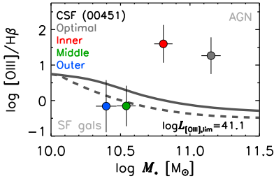
Figure 6. CSF’s resolved mass–excitation diagram (Juneau et al. 2014) at GLASS’s 2\sigma F_{\text{lim}} \simeq 2 \times 10^{-17} \text{ erg s}^{-1} \text{ cm}^{-2} (Schmidt et al. 2014; i.e., \log(L_{\text{O III}}/\text{erg s}^{-1})_{\text{lim}} = 41.1 ). INNER/optimal estimates imply AGN activity (above the solid line). Meanwhile, the MIDDLE and OUTER regions lie with normal star-forming galaxies (below the dashed line). These maintain a combined SFR \sim 10\text{--}25 M_{\odot} \text{ yr}^{-1} , apparently quenched by the AGN (Figure 4).
