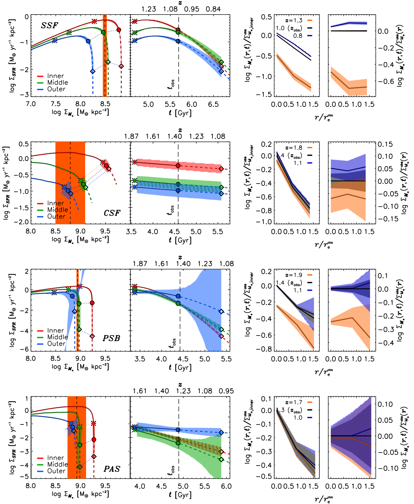
Figure 10. Resolved mass growth histories. From left: (1) \Sigma_{\text{SFR}}(r) vs. M_* surface density; (2) \Sigma_{\text{SFR}}(r) vs. cosmic time; (3) \Sigma_{M_*}(r) profiles at t_{\text{obs}} \pm 1 Gyr normalized to INNER values at t_{\text{obs}} (shape evolution); and (4) \Sigma_{M_*}(r) at the same epochs normalized to the observed profile (total M_* growth). Points in the left two panels denote epochs in the right two; orange vertical bars show INNER \Sigma_{M_*} at the time of peak INNER SFR. Shading shows 1\sigma ranges in all cases. All but CSF show signs of bulge-first growth, visible in the resolved \Sigma_{\text{SFR}}(t) , the change in rank ordering of \Sigma_{\text{SFR}}(M_*, t) , and the profile evolution itself. All but CSF (Section 5.1) suggest that INNER \Sigma_{M_*} at peak SFR is a kind of asymptote for the MIDDLE and OUTER regions, though the INNER regions themselves may \sim double since passing this mark. This trend may reflect a bulge-building–quenching association (Zolotov et al. 2015; Tacchella et al. 2016b; Figure 12, below) or a coincidence given the masses/mass profiles of these systems. Note that the confidence intervals at left reflect the fact that x = \int y , so (large) SFR errors propagate to mass.
