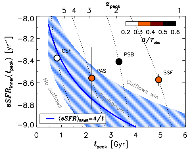
Figure 12. Higher B/T galaxies (point colors) had super-SFMS INNER sSFRs when their SFHs peaked and were always “overactive” according to their median SFH (dotted lines). Conversely, CSF has the lowest B/T and never rose above/had stayed near the SFMS, which was higher at CSF’s earlier peak time. If the SFMS reflects inflow/outflow equilibrium (e.g., Davé et al. 2011), this finding suggests a link between bulge building and a feedback-related mechanism turning SFHs over (outflows beat inflows; Zolotov et al. 2015; Tacchella et al. 2016b). Disk galaxies may therefore be objects with flat/quasi-constant SFHs (Figures 9 and 14; Sections 4.3.2, 5.1.2).
