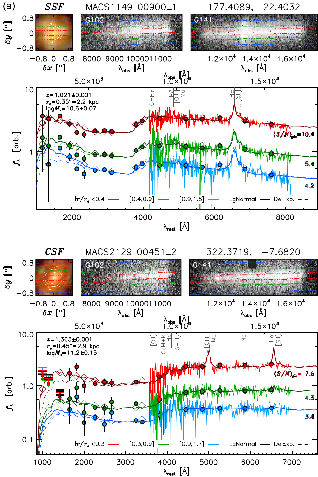
Figure 2. (a) Images, 2D spectra, and spatially resolved 1D extractions for SSF and CSF (others on next page). The top left images are insets of those in Figure 1 showing 1D r_e (solid) and 2D half-light radii (dashed circles), the extraction regions, and the light-weighted (x, y) centroids for each. Rightward of these are the 2D GLASS spectra with extraction zones overlaid in red (INNER), green (MIDDLE), and blue (OUTER). Steps are due to the spectra not being (x, y) rectified. Black areas on the 2D spectra show contamination/missing data masking. The main panel shows corresponding 1D SEDs color-coded by region. The best-fit pyspecfit lognormal (delayed exponential) SED fit is plotted as a solid (dashed) line, with open diamonds showing the predicted locations of the photometry. In all but PSB, the lognormal provides as good a fit to the data as the delayed exponential SFH. The radial extent of each extraction zone is listed at the bottom. (b) Images, 2D spectra, and radial 1D spectra for PSB and PAS.
