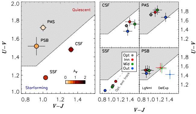
Figure 3. Left: synthetic integrated rest- UVJ colors color-coded by A_V . Consistent with appearances, CSF and SSF lie in the star-forming region and are more extinguished than their quiescent counterparts. Right: resolved colors from the radial spectral extractions. CSF and SSF have x or y gradients such that INNER regions are redder than OUTER ones. The quiescent PAS and PSB show opposite or no gradients (with the caveat of PSB’s limited radial coverage). SSF’s pieces lie roughly along the trajectory of its integrated SED fit, suggesting that larger- r regions developmentally lag INNER ones (“inside-out growth”). PSB is the only system with rest-frame color SFH systematics (both results plotted at bottom right), perhaps due to its truncated history or our lack of rest- J coverage (available only from insufficiently resolved Spitzer data).
