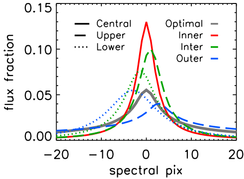
Figure 16. LSFs for CSF's unfolded radial and optimal extractions showing offsets and chord profile variations (Section 2.3). These preclude a priori impositions of symmetry in objects with PA \sim 45^\circ .
