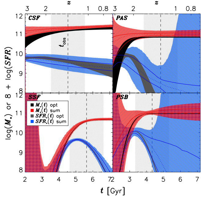
Figure 17. The SFHs and mass growth curves from the optimal integrated extractions (black/gray, respectively) vs. those summing INNER, 2 \times MIDDLE, and 2 \times OUTER results (blue/red, respectively). Vertical dashes show t_{\text{obs}} with the \pm 1 Gyr projection window shaded (Section 4.3.2). The 1\sigma summed uncertainties are calculated as a fraction of the median (shading) and as the log of the high/low linear \text{SFR}(t) or M_*(t) estimates (solid lines). The former leads to mostly unconstrained (future) summed uncertainties for PAS and PSB due to their low \text{SFR}(t_{\text{obs}}) . Even so, the largely independent sums of the parts and inferences from the whole broadly agree.
