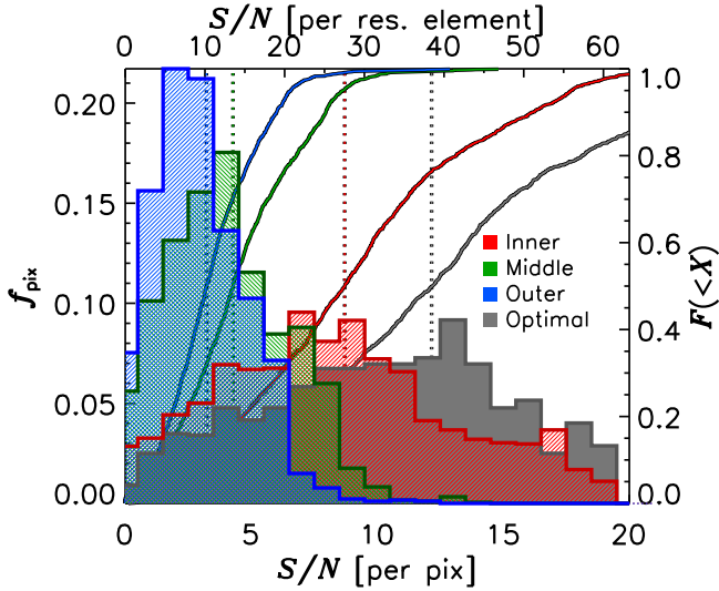
Figure 15. The S/N distributions for the 16 sample spectra (four per galaxy). INNER (red) covers |r/r_e| \lesssim 0.4 ; MIDDLE (green) and OUTER (blue) reach |r/r_e| \in (0.4, 1.0] and (1, 2] , respectively. Optimal extractions are plotted in gray. Dotted vertical lines show the median S/N.
