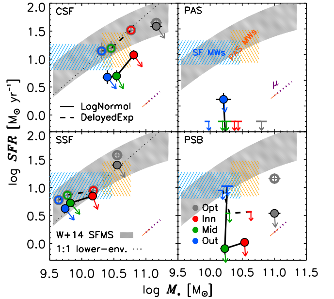
Figure 4. Spatially resolved SFR- M_* plane. Star-forming (passive) systems are plotted at left (right). Filled symbols/solid lines show lognormal results; open symbols/dashes show delayed exponentials. Bars denote 2\sigma upper limits; arrows are (M_*, SFR)(t) unit vectors averaged over t_{\text{obs}} \pm 1 Gyr. The z \sim 1.25 SFMS (Whitaker et al. 2014) is plotted in gray with blue/orange blocks locating progenitors of z = 0 MW-mass SF/passive galaxies (Gladders et al. 2013). Resolved and integrated metrics (colored and gray circles, respectively) support similar inferences with telling exceptions: the SFMS’s bend allows galaxies to be on the locus while their components are not (CSF), suggesting that locus-based inferences can bias insights into star formation physics. Dotted purple/thin orange lines show magnification effects/uncertainties.
