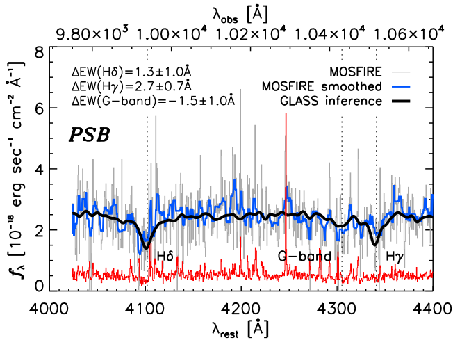
Figure 8. PSB’s optimal lognormal model spectrum (black; broadened to \sigma_v = 190 \pm 40 \text{ km s}^{-1} ) compared to MOSFIRE data (gray). Red shows rms errors, and blue shows median-smoothed data (10 Å window). Implied line strengths show that the lognormal SFH may reproduce these high spectral resolution data better than the delayed exponential, though the latter better matches PSB’s UV fluxes (cf. Table 3 and Figure 2).
