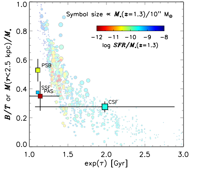
Figure 14. GLASS sample data inferences (squares) vs. G13 B/T - \tau predictions (circles; see main text and Abramson et al. 2016’s Figure 14 for details). Colors show model z = 1.27 = \langle z_{\text{GLASS}} \rangle and observed s\text{SFR} s. The data’s trend for higher measured B/T to correspond to smaller inferred \tau and the corresponding s\text{SFR} s is well predicted, though SSF and PSB are quantitatively low. This amplifies Section 5.1.2’s discussion of a bulge-growth/SFH shape connection—high (low) B/T implies SFHs that do (do not) turn over—a robust conclusion of this work and an independent consequence of G13 . Indeed, if CSF’s \tau error bar—and perhaps G13 ’s large- \tau tail—reflect the fact that they cannot formally be captured by a lognormal, this may suggest that galaxies with near-constant SFHs form a special class.
