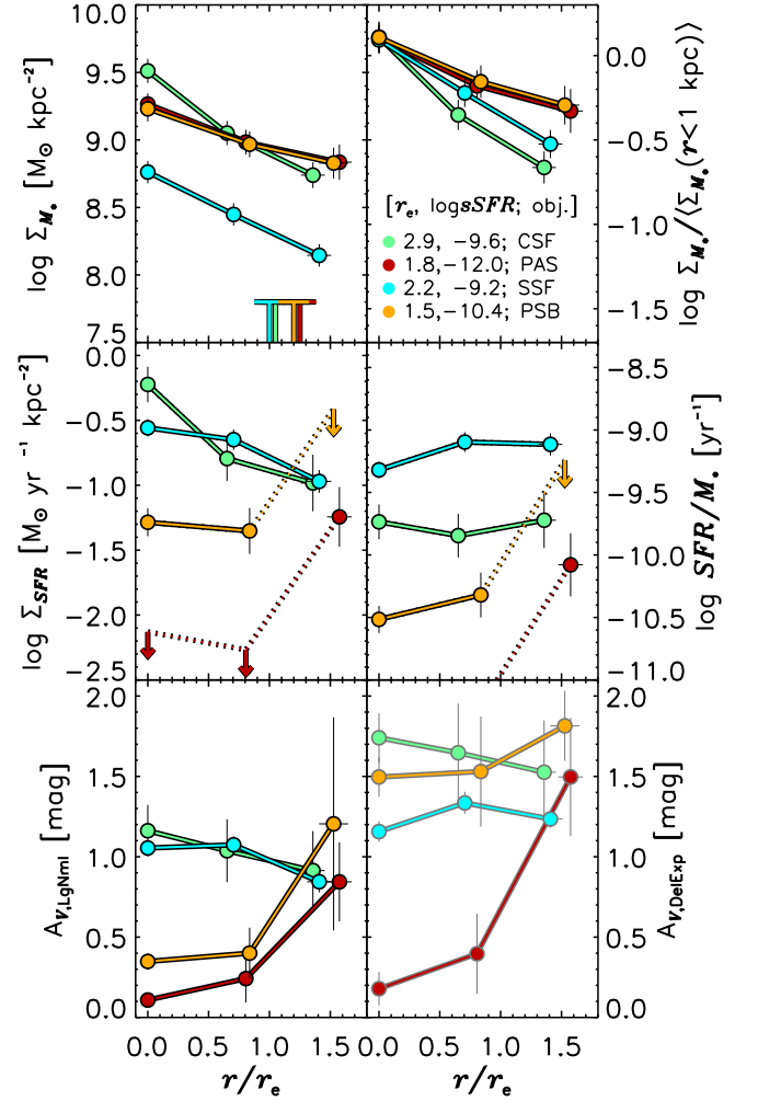
Figure 7. Top: lognormal absolute (left) and relative (right) mass surface density profiles. The latter are normalized to each source’s central kpc mean. Middle: SFR surface density and sSFR profiles (areas cancel). Bottom: A_V profiles from lognormal (left) and delayed exponential (right) SFHs. The sSFR ( r ) values of the star-forming systems differ by \sim 4\times , but they have consistent \Sigma_{\text{SFR}} at all r , favoring gas surface density over mass as an SFR governor. Here A_V exhibits SFH systematics, pointing to it as a test of SFH models (though the rest-UV S/N is low in the passive systems). Bin x offsets reflect pixelation.
