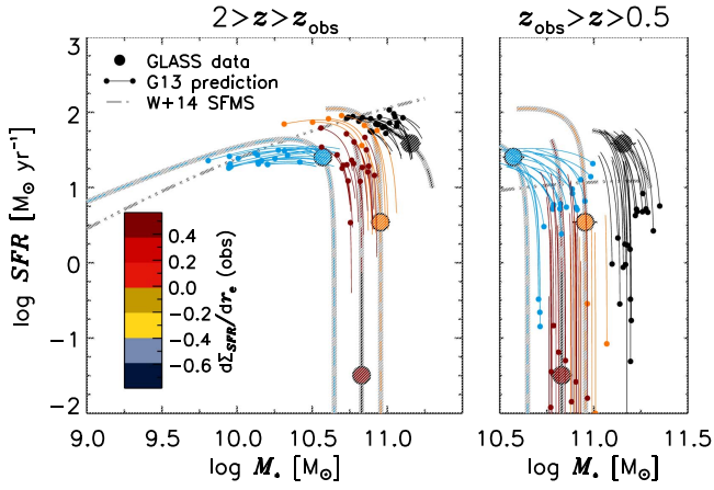
Figure 13. The G13 model SFHs (colored lines/small points) passing through the sample at t_{\text{obs}} (large points) projected to show progenitor/descendant envelopes at z = 2 (left) and 0.5 (right). Colors show \Sigma_{\text{SFR}}(r; t_{\text{obs}}) data slopes (Figure 7; bluer \rightarrow more negative). G13 generally captures the data-inferred SFHs, though SSF evolves faster than predicted; both agree that all systems were SFMS galaxies at z = 2 (gray dot-dashed lines; Whitaker et al. 2014), except possibly PAS, which may already have shut down. At z \sim 0.5 , CSF has an \sim 50\% chance of remaining a massive star-forming galaxy as data reconstructions suggest, while \sim 20\% of SSF’s tracks suggest that it will quench by then. More negative SFR gradients may imply slower evolution—another manifestation of bulge-first growth—but more data are needed to confirm.
