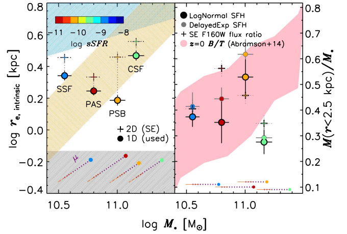
Figure 5. Left: the size–mass plane. Points are color-coded by sSFR with circles and crosses showing 1D r_e used in this analysis and 2D SExtractor half-light radii, respectively. Blue and orange shading shows van der Wel et al. (2014)’s star-forming and passive z = 1.25 relations, with the HST resolution limit in black. Right: the M_*(r < 2.5 \text{ kpc}) fraction ( \sim B/T )–mass plane with Abramson et al. (2014)’s z = 0 , 25%–75% range shaded pink (a good description at z \lesssim 2 ; Lang et al. 2014). Gray circles and dotted crosses show delayed exponential SFH and single-band SExtractor estimates to provide a sense of systematics. All galaxies have normal B/T for their mass except CSF, which is unexpectedly disk-dominated.
