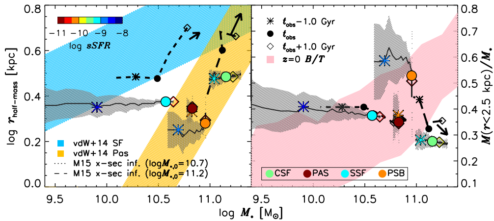
Figure 11. Same as Figure 5 but showing the longitudinally reconstructed half-mass-radius (left) and mass-concentration/ B/T -mass evolutionary trajectories of the sample galaxies. Black shading shows 1\sigma envelopes across 2 \geq z \geq 0.5 , with points denoting 1 Gyr before (asterisks) and after (diamonds) t_{\text{obs}} (filled circles). Point colors show s\text{SFR}(t) at the corresponding epochs. Short and long black dashes, respectively, show Morishita et al. (2015)’s cross-sectionally inferred trajectories for galaxies with the space densities of modern MW- and \gtrsim M31 -mass systems over the same z -range, highlighting the same intervals (referenced to \langle z \rangle = 1.27 ); arrows denote their time-averaged vectors. Population loci are shaded as in Figure 5. SSF, CSF, and PSB have all grown significantly in M_* since z = 2 , but not necessarily in size (cf. Genel et al. 2018). This behavior differs from cross-sectional inferences—even for CSF, whose mass evolution is well captured—but B/T inferences are more consistent, with galaxies tending to descend onto the fixed population locus with time from earlier states of relatively high B/T (inside-out growth). At left, note that three systems will end up as small red galaxies at z \sim 0.5 , though these will have gotten there in very different ways (Section 4.3.2), highlighting the importance of path dependence/temporal diversity underlying single-epoch parameter projections in galaxy evolution.
