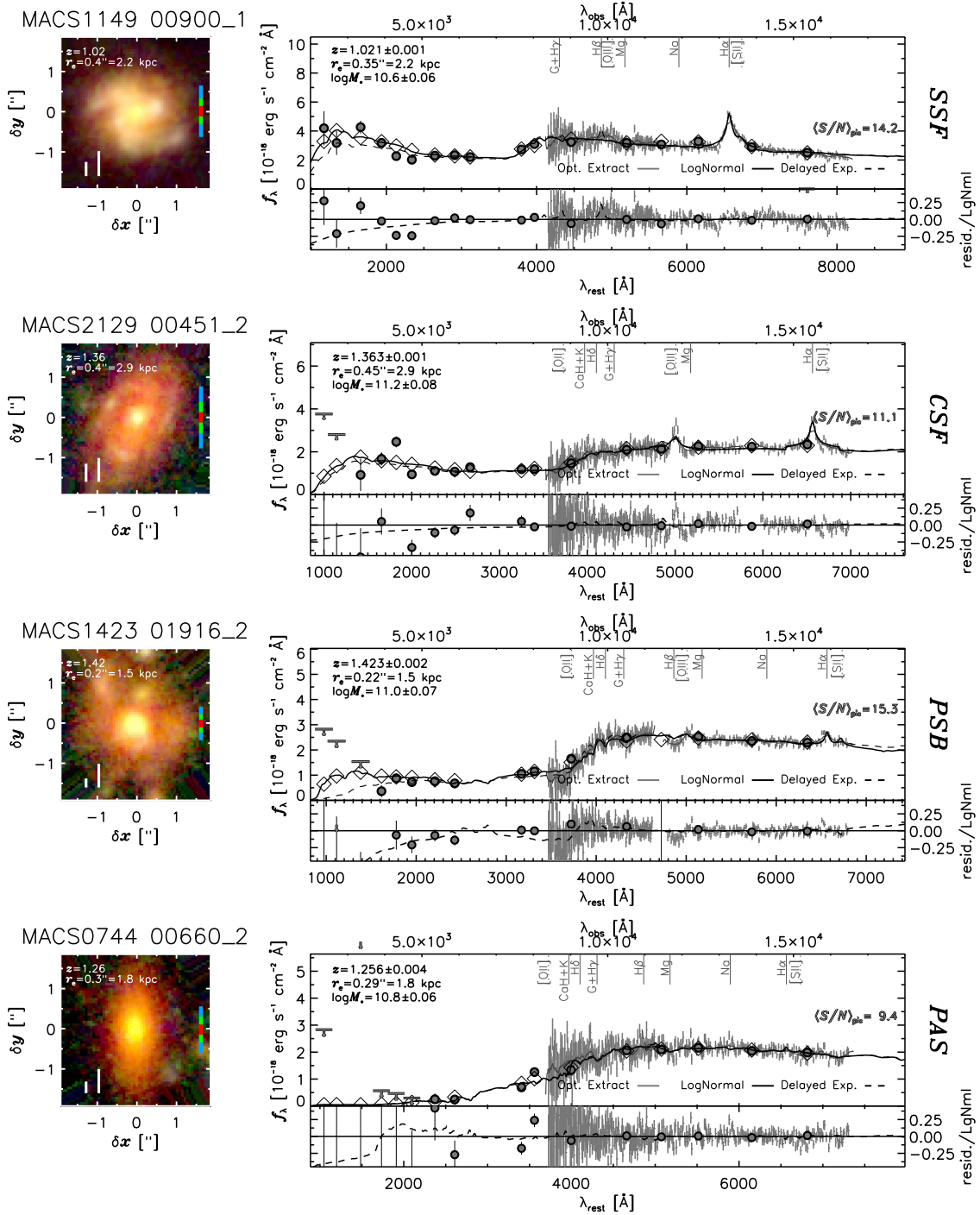
Figure 1. Color CLASH/HFF stamps and optimal GLASS spectra of the four sample objects (Table 1), ordered by decreasing sSFR from top to bottom. The smaller white scale bar on each \sim 4'' \times 4'' image shows r_e ; the larger shows 5 kpc at the source redshift. Multicolored scale bars at right show the location/width of the radial spectral zones (Section 2.3) color-coded as in Figure 2 and all further plots. CLASH/HFF photometry/ 2\sigma limits are denoted by circles and arrows, respectively, with open diamonds showing the pyspecfit model values assuming lognormal (solid) or delayed exponential (dashed lines) SFHs. Spectra are plotted as their 1\sigma uncertainty interval at each \lambda . Numbers at the red ends of the spectra give mean per-pixel S/N. Other integrated physical parameters are listed at the top left.
