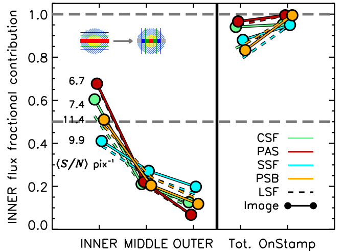
Figure 18. Contributions to the INNER regions’ spectra from all regions (assuming y \mapsto x symmetry; see inset cartoon). This is a metric of how closely our chord-based extraction ( y \sim 0 ) mimics a true radial one ( r \sim 0 ). INNER light dominates this slice in all objects but SSF, where it contributes 35%–40%. However, per-pixel S/N is sufficient to grant \geq 1.5\sigma purchase on the effect of this plurality contribution, which manifests in SSF’s clear signs of differential central/outskirts growth (e.g., Figure 10). Lateral contamination makes such inferences a lower limit. Conversely, the spatial uniformity of CSF’s SFHs should not be a result of INNER contamination given its INNER-INNER region’s majority contribution. The three zones capture 80%–95% of the total flux, with >95\% contained in the GLASS postage stamps.
