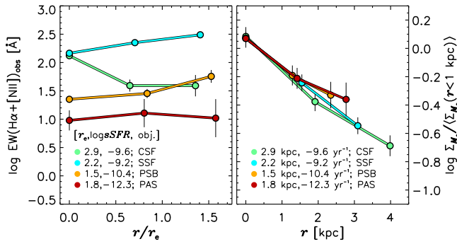
Figure 20. Reinterpretations of Figure 7. Left: dust-uncorrected \text{EW}(\text{H}\alpha + [\text{NII}]) yields similar trends to SED-fit sSFRs. CSF is an exception: AGN activity elevates the INNER inference (Figures 2 and 6), while those at larger r are \sim 10\times depressed relative to SSF. The IFU data will reveal if this is due to increased extinction toward CSF’s H II regions or a real suppression of sSFR beyond the factor of \sim 3 inferred from the full SED. Right: inner kpc-normalized \Sigma_{M^*} profiles vs. physical radii (as opposed to r/r_e ), highlighting the sample galaxies’ sizes. Trends are the same as in the main-text figure, with the larger star-forming systems having steeper mass profiles than the passive ones, perhaps suggesting that the latter already have some dry merging (Section 4.2; e.g., Newman et al. 2012).
