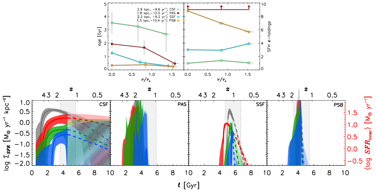
Figure 19. Summary plots based on the delayed exponential SFH fits (Section 3). The top panels show radial parameter trends—age \equiv t_{\text{obs}} - t_{\text{start}} , e -foldings = age/ \tau_{\text{exp}} —that reveal similar signatures of inside-out growth to the main lognormal analysis (INNER regions older/having undergone more e -foldings). The bottom panels reproduce Figure 9, showing the SFHs in full. These qualitatively reflect the lognormal results for CSF’s and SSF’s INNER region, but PSB and PAS become essentially a convolution of \delta -functions, implying unrealistic growth rates in PSB’s case and forbidding time-domain reconstructions. Note that inferences such as the INNER/OUTER SFH crossing epoch (inside-out transition) in SSF agree using either method (cf. Figure 10).
