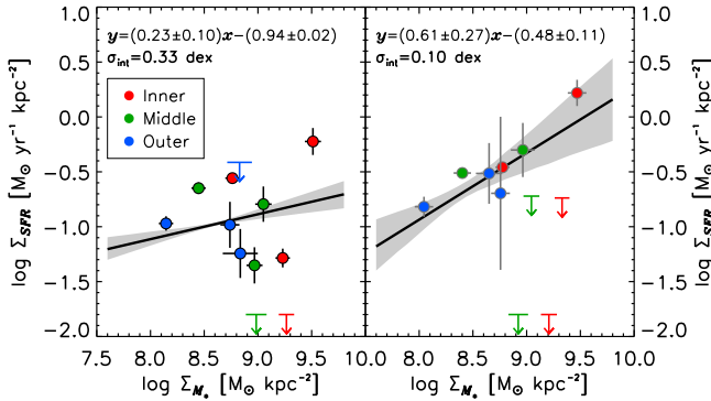
Figure 21. Resolved SFR vs. M^* surface densities (analogous to Schmidt 1959; Kennicutt 1998) assuming lognormal (left) and delayed exponential SFHs (right). Both have x \equiv \log \Sigma_{M^*} - 8.75 , with linear best fits performed only to detections by bootstrapping and varying points by their x and y error bars. While quite different from each other, both inferences are similar to z = 0 IFU/resolved SED estimates over a similar mass (but not \Sigma_{M^*} ) range: Cano-Díaz et al. (2016) found a slope/dispersion of 0.68 \pm 0.04 and 0.23 dex, respectively, corresponding to our delayed exponential results; Abdurro’uf & Akiyama (2017) found 0.33 and 0.7, respectively, closer to our lognormal results. This highlights the dependence of scaling relations on SFH choice.
