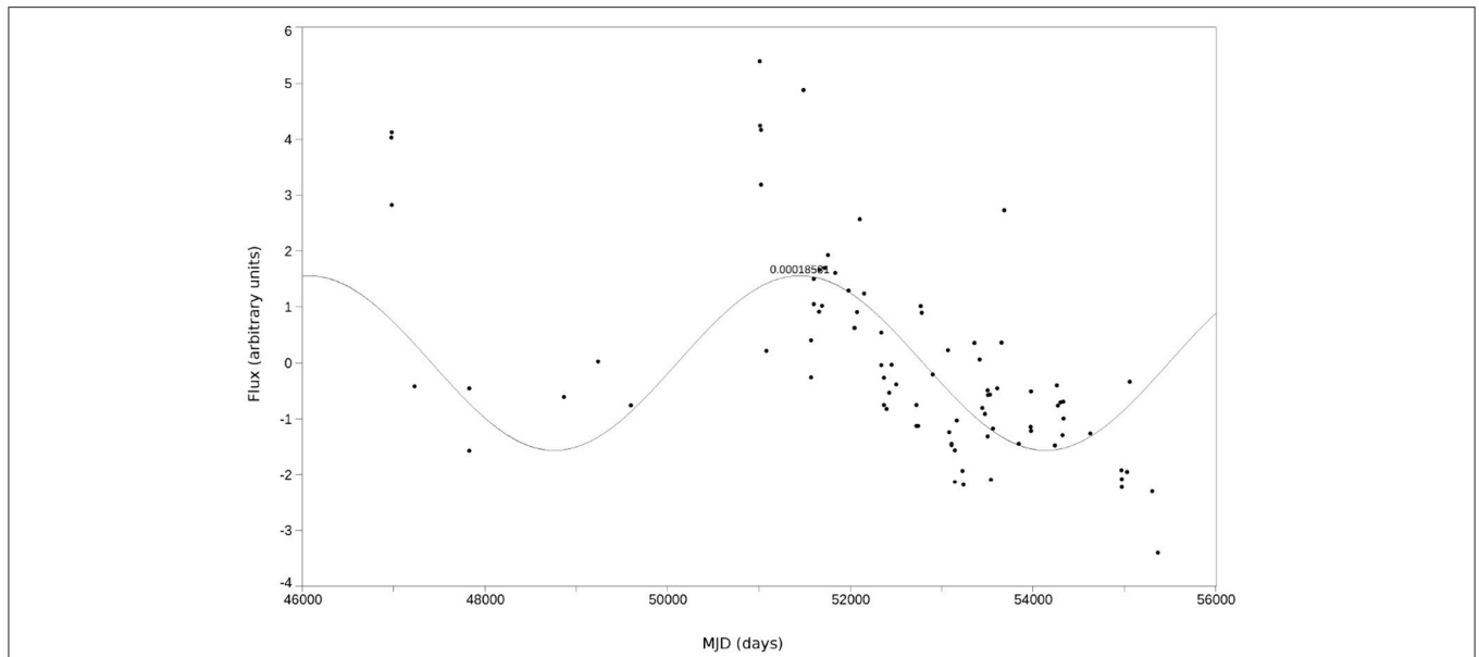
FIGURE 3 | Long term variability analysis of Arp 102B light curve after trend removal correction fitted with the sine function with the period of about 14 years.
