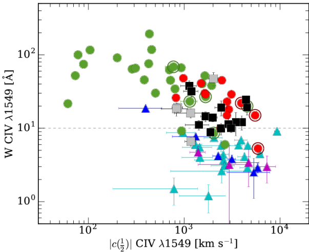
Fig. 10. Relation between rest-frame equivalent width of \text{CIV}\lambda 1549 and c(\frac{1}{2}) in \text{km s}^{-1} . Black squares: GTC-xA. Gray squares: BAL GTC-xA. Blue triangles: Plotkin et al. (2015), magenta: Wu et al. (2012) and cyan: Luo et al. (2015). Red and green circles correspond to the Pop. A samples from S17 and FOS-A sample, respectively. Circled symbols correspond to FOS-xA and S17-xA.
