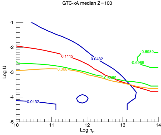
Fig. 7. Isocontours in the plane \log of ionization parameter ( U ) versus \log of hydrogen density ( n_{\text{H}} ) from CLOUDY simulations for the line intensity ratios \text{AlIII}\lambda 1860/\text{SiIII}\lambda 1892 (blue), \text{HeII}\lambda 1640/\text{CIV}\lambda 1549 (green), \text{CIV}\lambda 1549/\text{AlIII}\lambda 1860 (yellow), \text{CIV}\lambda 1549/\text{SiIII}\lambda 1892 (red) using Z = 100Z_{\odot} . Labels report the median values of the intensity ratios for the objects of the GTC-xA sample.
