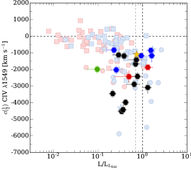
Fig. 9. Behavior of the centroid at 1/2 of total \text{CIV}\lambda 1549 profile as a function of Eddington ratio. Hexagons represent the GTC-xA sample. The colors of hexagons are the same as Figures 2 and 3. Blue and red pale symbols correspond to the Population A and B, respectively. Squares and stars correspond to the FOS-A and xA samples (Sulentic et al. 2007). Circles are from HE sample Sulentic et al. (2017) sample. Yellow star marks the position of I Zw 1. The black dashed horizontal line indicates c(\frac{1}{2})=0 \text{ km s}^{-1} . Gray and black dashed vertical lines indicate L/L_{\text{Edd}}=0.2 and 1.0, respectively.
