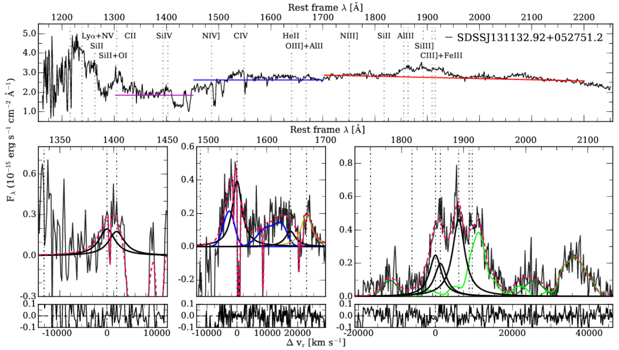
Fig. A.11. (cont.) Same of the previous panel, for SDSSJ131132.92+052751.2.
