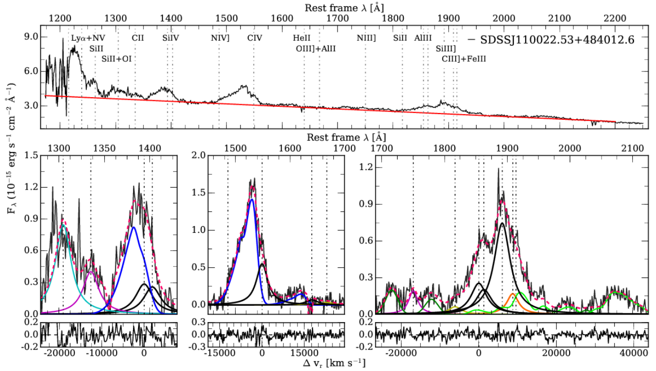
Fig. A.9. (cont.) Same of the previous panel, for SDSSJ110022.53+484012.6.
