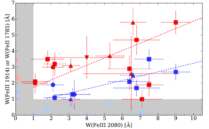
Fig. 8. Relation between intensity of the \text{FeIII} feature at 2080 Å with \text{FeII} UV 1785 Å (blue) and \text{FeIII}\lambda 1914 (red). Squares, up and down triangles, and circles mark the normal, BAL, mini-BAL and RL quasars, respectively. The gray shaded area indicates an approximate detection limit. Blue and red lines mark the orthogonal fit for each case.
