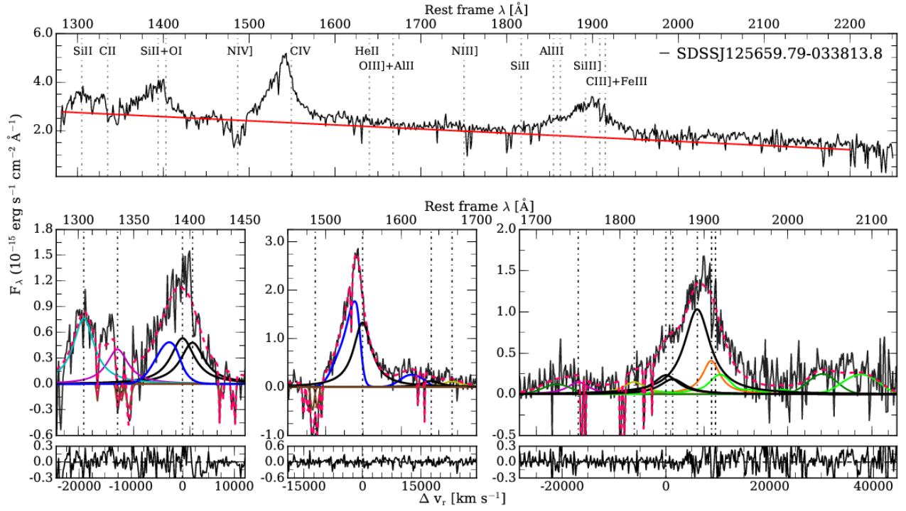
Fig. A.10. (cont.) Same of the previous panel, for SDSSJ125659.79-033813.8.
