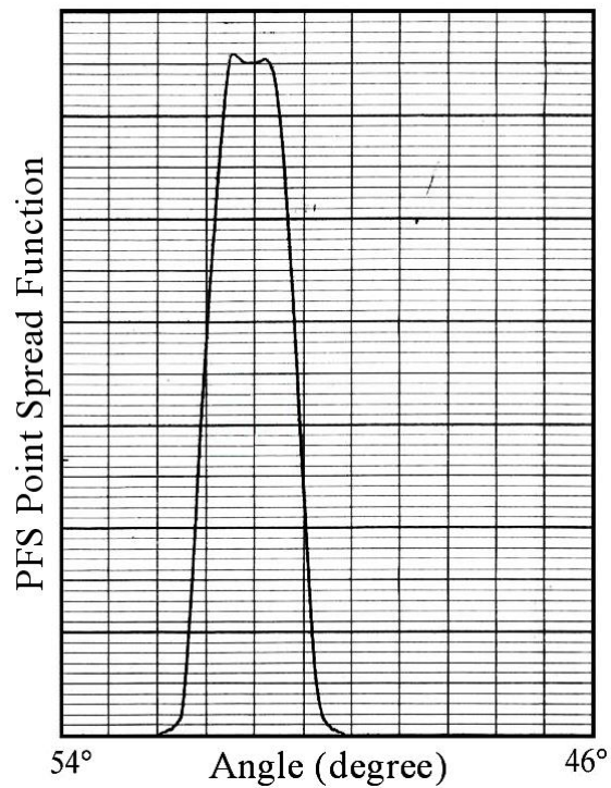
Figure A1. The PFS Point Spread Function measured in the laboratory. Note the steepness of the function and the plateau on the top.
