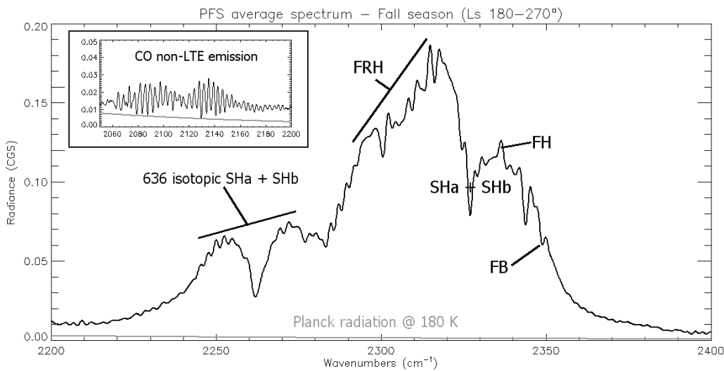
Figure 3. An average of about 3000 PFS limb spectra, selected during the southern spring ( 180^\circ < \text{Ls} < 270^\circ ), in the southern hemisphere (latitude < 0^\circ ), and for tangent altitudes between 50 and 200 km. Several emission bands can be easily identified in the spectrum. FB, FH, SH, TH, and FRH mean fundamental, first hot, third hot, and fourth hot bands, respectively. The small top-left panel shows the CO emission spectrum at 4.7 \mu\text{m} for the same average. The gray curve is the Planck radiation at 180 K.
