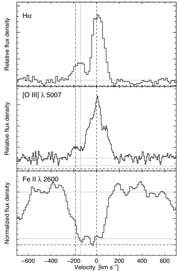
Figure 8. The velocity profiles of the H \alpha and [O III] \lambda 5007 emission lines (top and middle) and the normalized low-ionization absorption lines represented by Fe II \lambda 2600 (bottom). The respective error spectra are overlaid as the dotted lines. The zero-point of the velocity scale is set to the systemic redshift of z = 0.73696 (dashed line) measured from the emission lines. The dotted and dash-dotted lines show the centroid of the two blueshifted components seen in emission from H \alpha and [O III], respectively.
