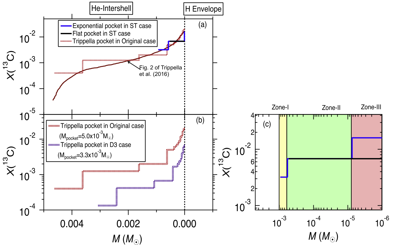
Figure 2. ^{13}\text{C} mass fraction ( X(^{13}\text{C}) ) is plotted against the stellar mass in units of M_{\odot} proceeding from the bottom of the H-envelope (right) to the He-intershell (left) of an AGB star. The stellar mass coordinate at the interface of the two layers is defined as zero. Different ^{13}\text{C} profiles are explained in the text and shown as different colored lines. A smaller Trippella pocket ( 3.3 \times 10^{-3} M_{\odot} ) in the D3 case, which might arise from a weaker magnetic field or interactions between magnetic and hydrodynamic effects, is shown in (b) to illustrate how the mass fraction and the mass extension are varied in Torino models to test their effects on s -process model predictions. The three zones of the Exponential ^{13}\text{C} -pocket are labeled in yellow (Zone-I), green (Zone-II), and red (Zone-III) in (c) in logarithmic scale.
