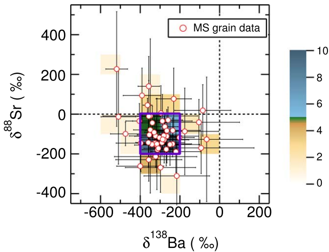
Figure 3. Four-isotope plot of \delta^{88}\text{Sr} vs. \delta^{138}\text{Ba} values for presolar MS SiC grains from Liu et al. (2015) and Stephan et al. (2018). The 2D joint histogram of the data is shown using a yellow-to-blue color scheme to reflect the grain density, and the number next to the color scheme represents the corresponding number of grains. The grain-concentrated region is highlighted by a purple box.
