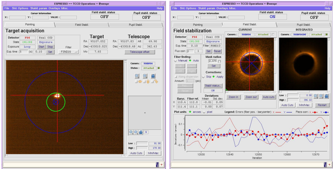
Figure 4: ESPRESSO operational GUI with tab activated for the pointing phase (left) and stabilization phase (right); see text for a detailed description.
