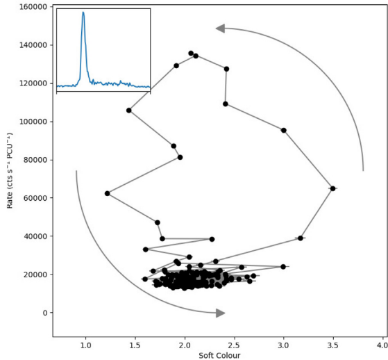
Figure 11. A 1 s-binned hardness-intensity diagram of a Normal Burst from RXTE/PCA observation 10401-01-08-00, with an inset 2–60 keV light curve. Significant colour evolution can be seen during the burst, taking the form of a loop.
