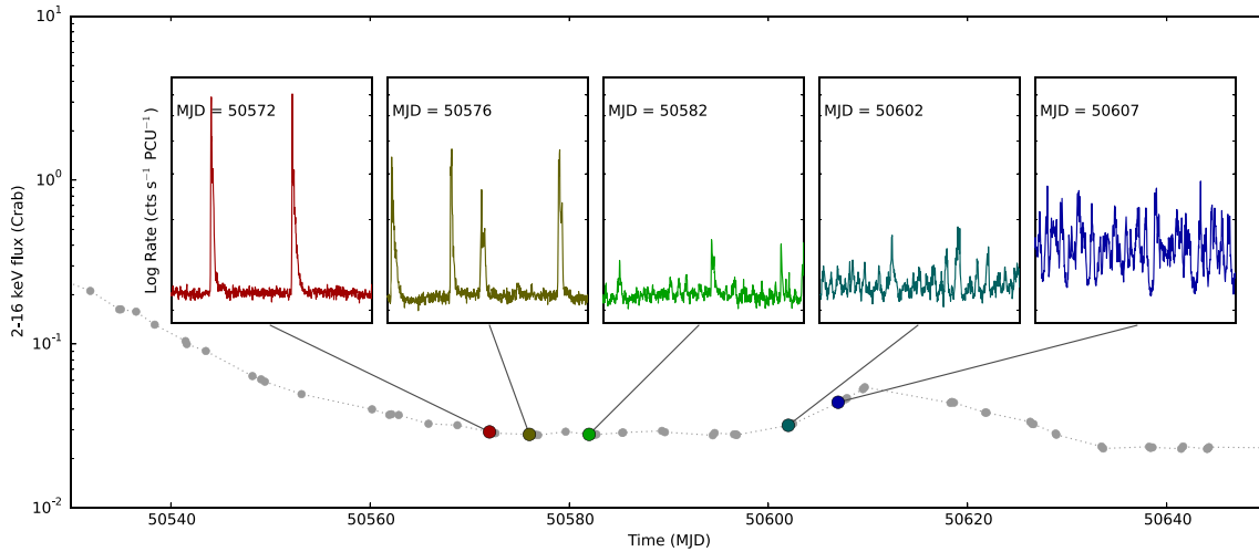
Figure 20. A series of light curves from RXTE/PCA observations of Outburst 2, showing a gradual evolution from Mesobursts to Structured Bursting over a period of \sim 30 d. Each inset light curve is plotted with the same y-scaling, and each corresponds to 2 ks of data.
