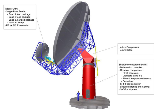
Figure 1: SKA DISH overview.
