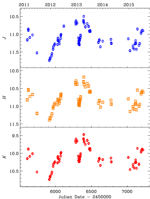
Figure 2. Near-IR light curves of Mrk 421 built with data from the GASP-WEBT collaboration in J , H and K bands. No correction for the host-galaxy contribution and Galactic extinction has been applied.
