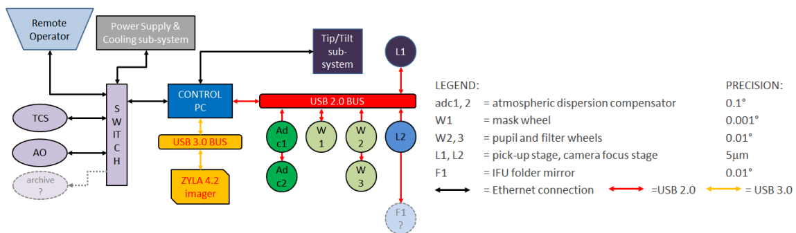
Figure 8: V-SHARK control architecture. Precision requested to the hardware devices are on the right side of the legend.
