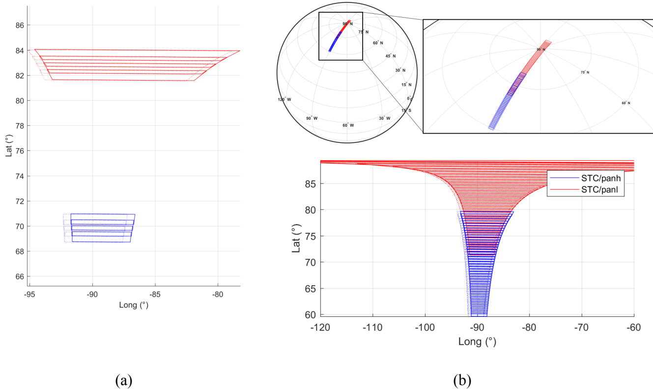
Figure 12 STC-PANH and PANL FoV projection on the Mercury surface at aphelion 0 orbit around sub-nadir latitude +83^\circ (polar region). On-ground FoV projection for 2 consecutive orbits on the surface of Mercury of the panchromatic filters of SIMBIOSYS STC -H and -L (respectively in blue and red). In (a) simulation of 4 consecutive acquisitions with a repetition time of 10 s (which around the poles guarantees the along track overlapping). Cross track overlapping is almost complete. In (b) same simulation but extended to 7 minutes projected on the Mercury sphere (upper images) and with the equirectangular projection (bottom image).
