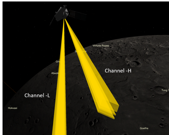
Figure 8 Screenshot of Cosmographia Tools showing the two sub-channels FoVs of STC. For the sub-channel-H, it is possible to note the FoVs of the Panchromatic filter (greater one) and the 2 colour filters.
