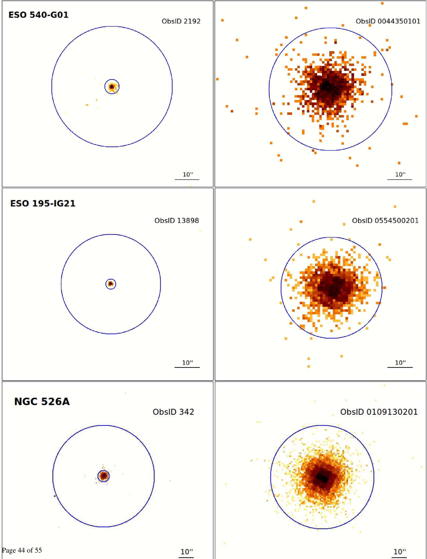
Fig. C.16: Images for Chandra data (left) and XMM-Newton data (right) for the sources in the 0.5-10 keV band. Big circles represent XMM-Newton data apertures. Small circles in the figures to the left represent the nuclear extraction aperture used with Chandra observations (see Table .1).
