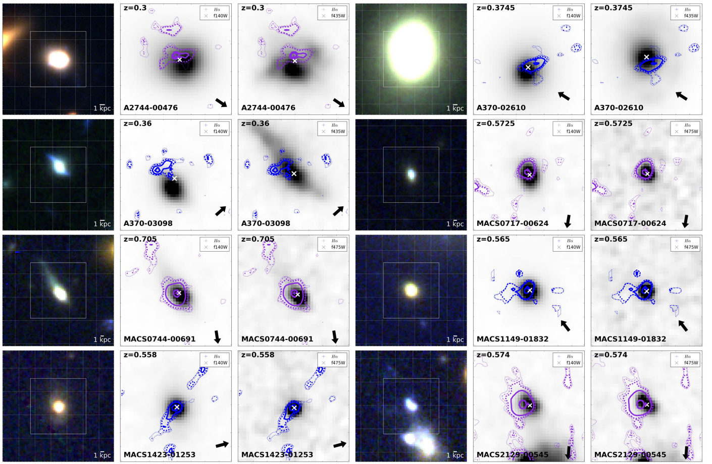
Figure 19. Cluster galaxies labeled as ram-pressure stripping candidates according to our classification scheme (Section 3.6). For each galaxy, the left panel shows the color composite image of the galaxy based on the CLASH (Postman et al. 2012) or HFF (Lotz et al. 2016) HST data. The blue channel is composed by the F435W, F475W, F555W, F606W, and F625W filters, the green by the F775W, F814W, F850lp, F105W, and F110W filters, and the red by the F125W, F140W, and F160W filters. The central panel shows the H\alpha map superimposed on the image of the galaxy in the F140W filter and the right panel shows the H\alpha map superimposed on the image of the galaxy in the F475W filter. Contour levels represent the 35th, 50th, 65th, 80th, and 95th percentiles of the light distribution, respectively. Blue contours indicate that H\alpha maps are obtained from one spectrum, purple contours indicate that H\alpha maps are obtained from two orthogonal spectra, and green contours indicate that H\alpha maps are obtained combining both the G102 and G141 grisms (only for z > 0.67 ). In the color composite image, the field of view is twice as big as the single-band images. A smoothing filter has been applied to the maps and an arbitrary stretch to the images for display purposes. Arrows on the bottom right corner indicate the direction of the cluster center. The redshift of the galaxy is indicated on the top left corner.
