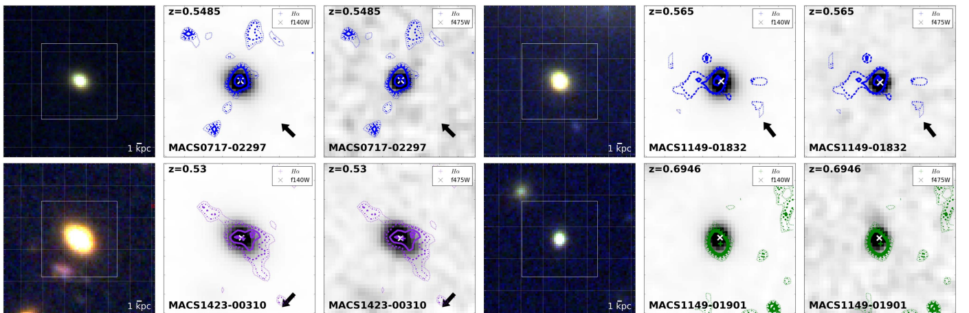
Figure 10. Example of galaxies with elliptical broad band morphology and detected H \alpha emission. For each galaxy, the left panel shows the color composite image of the galaxy based on the CLASH (Postman et al. 2012) or HFF (Lotz et al. 2016) HST data. The blue channel is composed by the F435W, F475W, F555W, F606W, and F625W filters, the green by the F775W, F814W, F850lp, F105W, and F110W filters, and the red by the F125W, F140W, and F160W filters. The central panel shows the H \alpha map superimposed on the image of the galaxy in the F140W filter and the right panel shows the H \alpha map superimposed on the image of the galaxy in the F475W filter. Contour levels represent the 35th, 50th, 65th, 80th, and 95th percentiles of the light distribution, respectively. Blue contours indicate that H \alpha maps are obtained from one spectrum, purple contours indicate that H \alpha maps are obtained from two orthogonal spectra, and green contours indicate that H \alpha maps are obtained by combining both the G102 and G141 grisms (only for z > 0.67 ). In the color composite image, the field of view is twice as big as the single-band images. A smoothing filter has been applied to the maps and an arbitrary stretch to the images for display purposes. For galaxies in clusters, arrows on the bottom right corner indicate the direction of the cluster center. The redshift of the galaxy is indicated on the top left corner.
