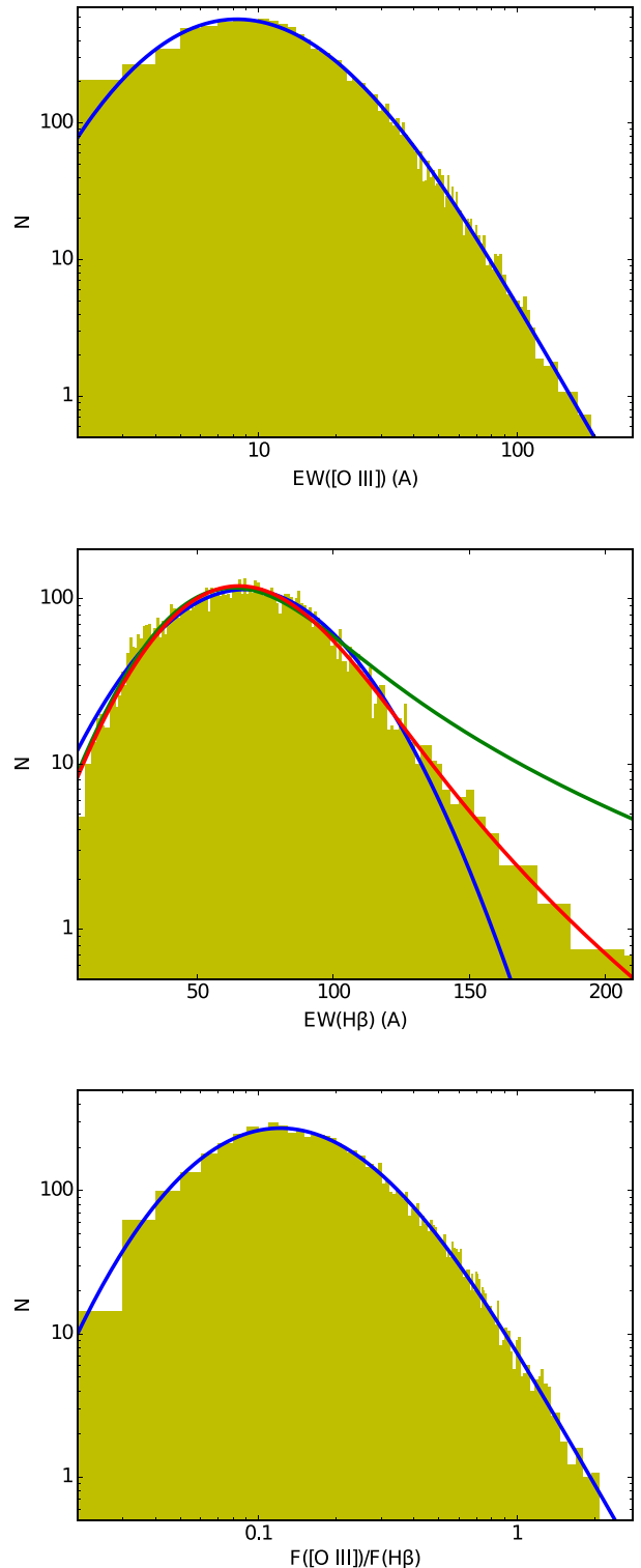
Figure 1. Observed distribution, and best-fitting curves, for (A) EW_{[O\text{ III}]} ; (B) EW(H\beta) ; (C) F([O\text{ III}])/F(H\beta) . The curves in panels B show the best fit with a high-EW tail slope \Gamma = 3.5 (green curve), a free slope (red curve; the best-fitting value is \Gamma = 6.9 \pm 0.2 ), and no tail (blue curve).
