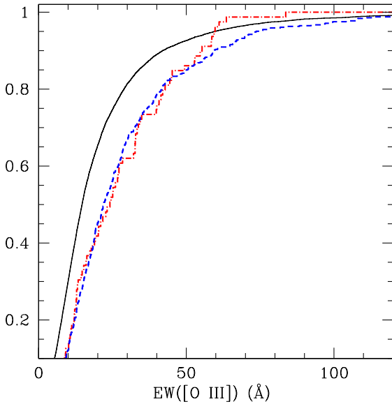
Figure 9. Cumulative distributions of EW_{[\text{O III}]} for the whole sample (black, continuous line), the ‘unambiguous’ double-peaked quasars (red, dot-dashed), and the ‘possible’ double-peaked quasars (blue, dotted line).
