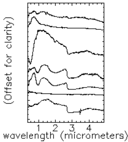
Fig.3 Spectral classes found in DAG489 slab
