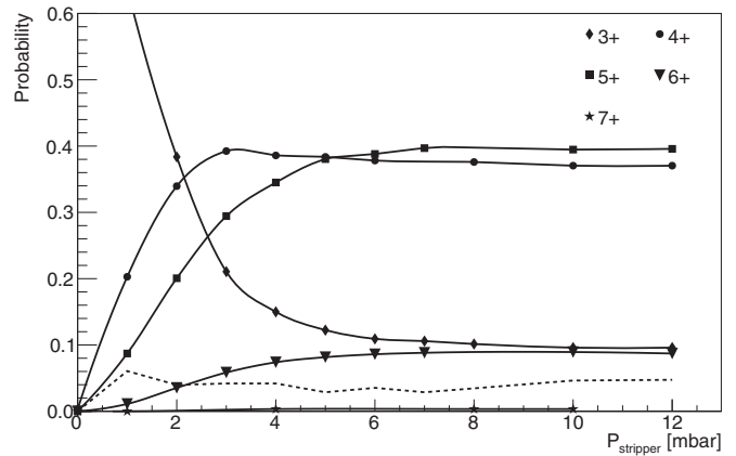
FIG. 4. Charge state probability of {}^{19}\text{F} ions as a function of the Ar post-stripper inlet pressure P_{\text{stripper}} at 5.0 MeV beam energy. Lines connecting the points are to guide the eye only. The dotted line represents the unmeasured current at this energy, due to nonaccessible 1+ , 2+ charge states and further charge exchanging in the CSSM chamber; see text for details.
