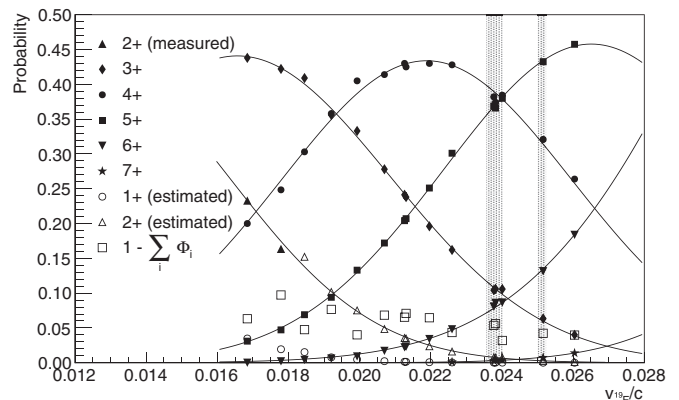
FIG. 5. Charge state probability of {}^{19}\text{F} ions determined by the Ar post-stripper as a function of velocity. Filled symbols are experimentally determined values, while empty symbols are estimated values for the unmeasured 1+ , 2+ charge states and for the further charge exchanging in the CSSM chamber; see text for details. Curves through points are uncorrelated Gaussian fits. Vertical shaded areas indicate the energy intervals where cross section measurements were performed.
