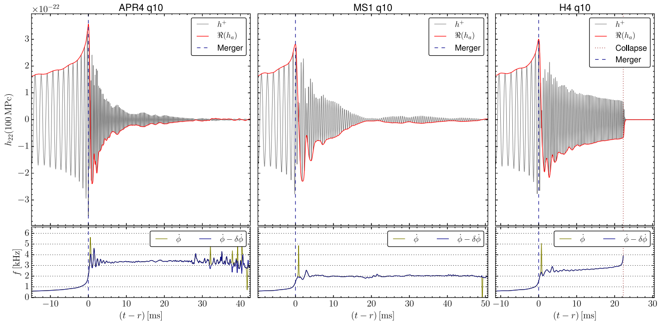
FIG. 24. Gravitational wave signal for the equal-mass APR4, MS1, and H4 models (from left to right). Top panels: the thin gray lines show the strain amplitude h_{22}^{+} at 100 Mpc, the red line the real part of the complex amplitude h_a (see text). Bottom panels: the phase velocity of the complex strain h_{22} before and after correcting for phase jump contributions (in yellow and blue, respectively). Note the phase velocity after 30 ms is not meaningful due to the low amplitude and lack of a clearly dominant mode. The vertical lines mark the times of merger (dashed) and of black hole formation (dotted).
