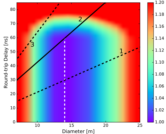
Figure 13. The background coloring with colorbar shows the relative cost/performance for delay and cost at a fixed performance as a function of element diameter. See §4.3, §4.4 and DeBoer & Parsons (2015) for details. A diameter of 14-m (vertical dashed line) is near the cost minimum and consistent with assumptions for the delay specification.
