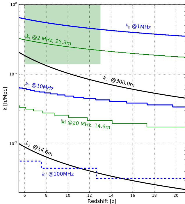
Figure 11. |\mathbf{k}| , k_{\parallel} , k_{\perp} wavenumber plots at various bandwidths ( k_{\parallel} ; blue), baselines ( k_{\perp} ; black), and total ( |\mathbf{k}| , green) as a function of redshift. The stepped profiles for k_{\parallel} and |\mathbf{k}| are the line-of-sight redshift ranges for that bandwidth (too small to see at 1 MHz). See text for discussion. The full redshift range is the HERA extended goal. The initial HERA delay-spectrum power spectrum goal is the light green square region in the upper left.
