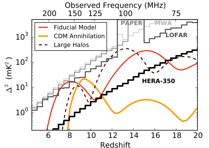
Figure 4. 1\sigma thermal noise errors on \Delta^2(k) , the 21 cm power spectrum, at k=0.2 h \text{ Mpc}^{-1} (the dominant error at that k ) with 1080 hours of integration (black) compared with various heating and reionization models (colored). Sensitivity analysis is per Table 1 and associated text.
