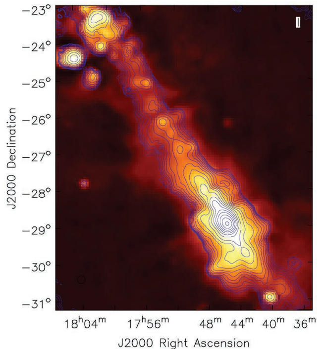
Figure 8. The color-scale shows an input model image of the Galactic center region based on the Effelsberg 21cm continuum survey (Reich et al. 1990). The contours show the mock HERA-350 observation at 130MHz with a resolution of 12' . Contour levels are a geometric progression in square root 2, starting at 5 \text{ Jy beam}^{-1} . The peak surface brightness on the HERA image is 2330 \text{ Jy beam}^{-1} .
