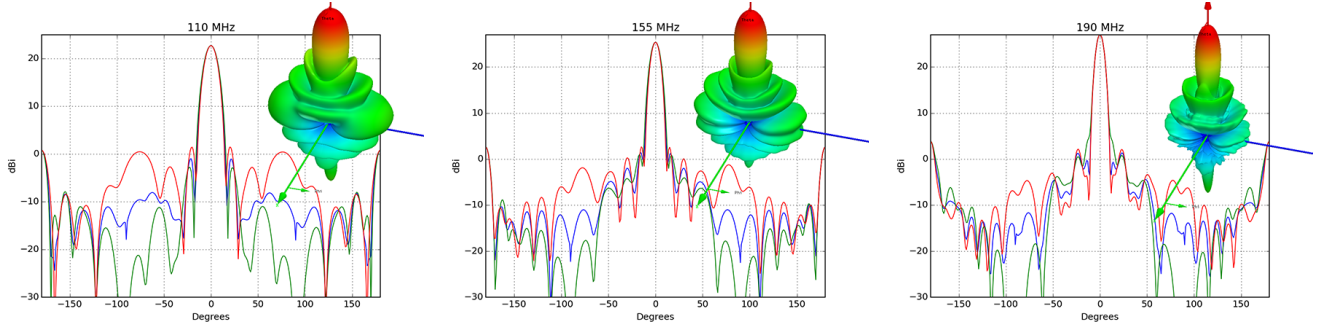
Figure 19. Antenna patterns at 110 MHz, 155 MHz and 190 MHz calculated with HFSS and the adopted design. Red curves are E-plane, green are H-plane at blue at 45^\circ . Inset is the full 3D pattern.
