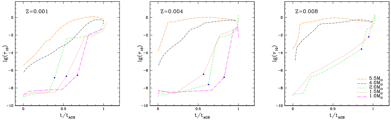
Figure 2. The variation during the AGB evolution of the optical depth, \tau_{10} , of AGB models of different initial mass and metallicity Z = 10^{-3} (left-hand panel), Z = 4 \times 10^{-3} (middle) and Z = 8 \times 10^{-3} (right-hand panel). Times on the abscissa are normalized to the total duration of the AGB phase. Blue squares along the tracks mark the beginning of the C-star phase. In the right-hand panel, we do not show 1 M_{\odot} model at Z = 8 \times 10^{-3} , which does not become a C-star.
