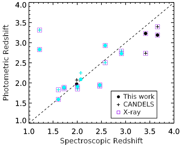
Figure 5. Spectroscopic redshift versus photometric redshift for galaxies in our sample. 24 \mu\text{m} -detected galaxies are denoted in cyan while X-ray sources are denoted by purple open squares. Both photometric redshifts derived using FAST in this work and those from CANDELS are presented.
