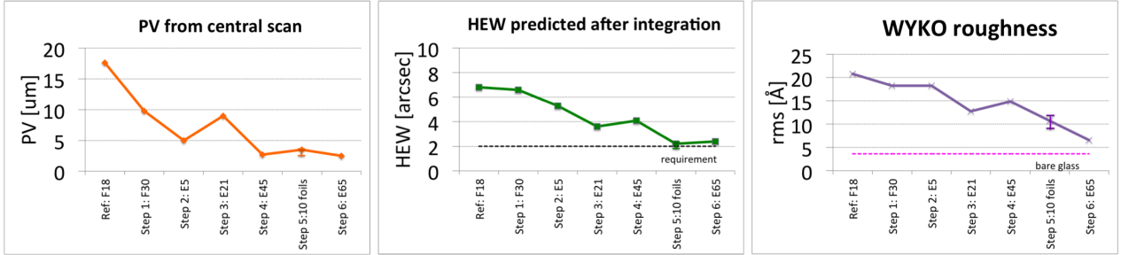
Figure 8. : Trend of three figures of merit selected to describe the reduction of the low- mid- and high- frequency errors of the glass foils slumped to cylindrical shape and integrated with ribs to Wolter I shape, for the IXO/ATHENA application as developed at INAF-OAB. Left: PV of the central LTP scan, the most critical as the less corrected during the integration with ribs. Center: HEW values expected from the LTP slumped glass profiles, obtained with physical optics 28 in single reflection after the simulation of a perfect integration. Right: roughness from the WYKO data.
