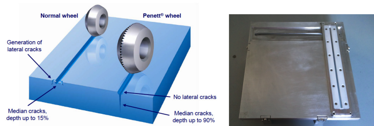
Figure 11. : Left: the MDI Penett's wheel, credits: MDI. Right: the template used at INAF-OAB to cut the slumped glass foils: the template has a bottom surface cylindrically shaped to follow the cylindrical cutting mandrel.
