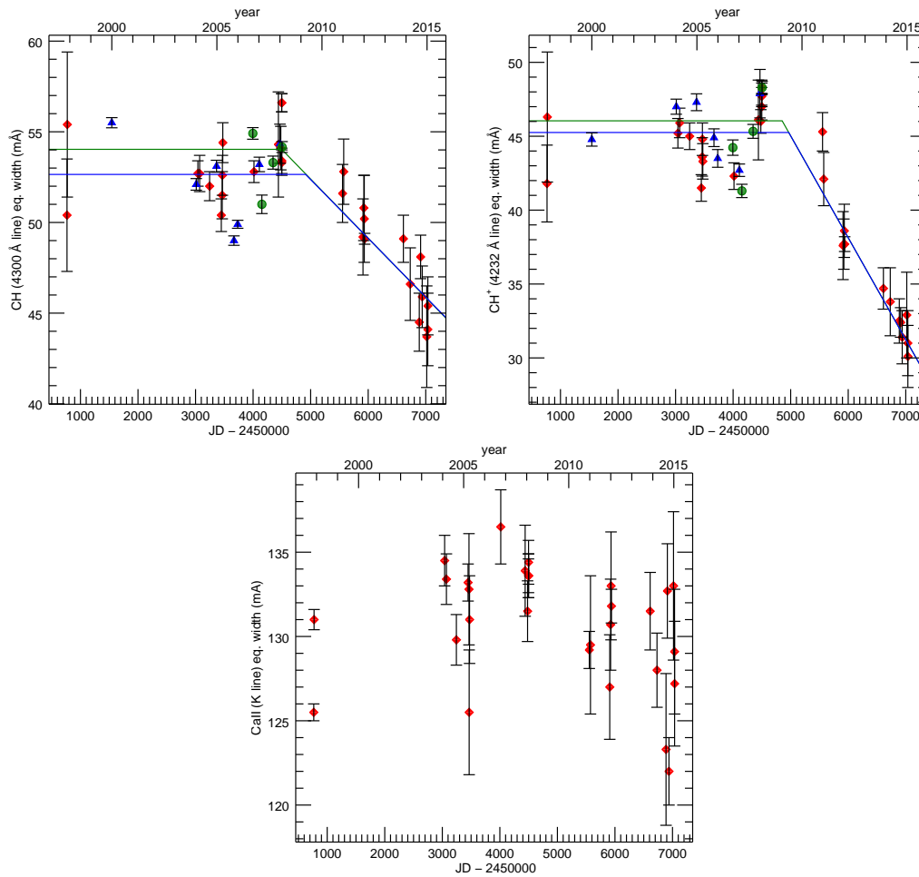
Fig. 2. CH 4300 Å, CH + 4232 Å, and CaII K line intensities plotted as a function of the observation epoch (in Julian days). The CH + decline is evident while that of CH is smaller. Red dots are our measurements, blue dots and green dots are respectively McDonald and OHP-SOPHIE observations, both from Boissé et al. (2009).
