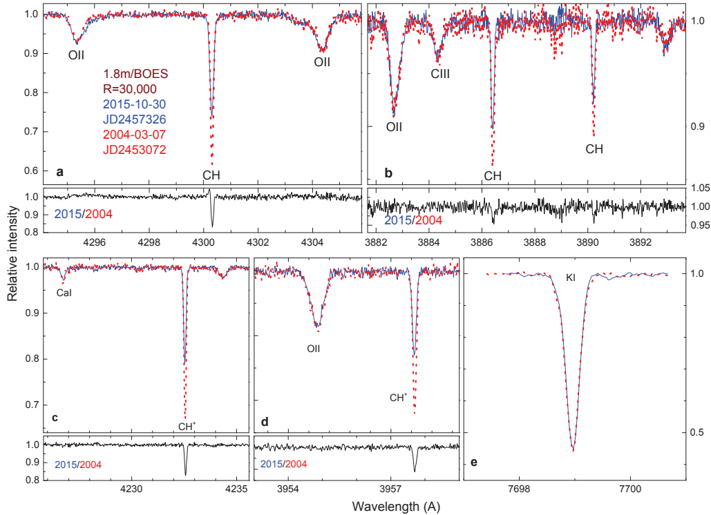
Fig. 1. Comparison between observations made in different epochs using the same instrument. Molecular lines are evidently weaker in the recently recorded spectrum in a sharp contrast to stellar lines and the interstellar CaI and KI ones.
