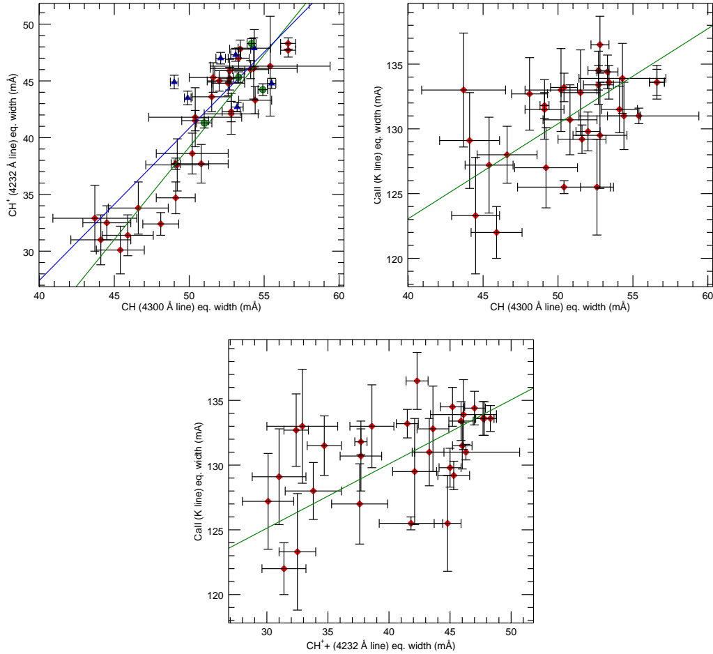
Fig. 3. Correlation plots of the EWs of CH, CH + and CaII. Left top panel : CH vs. CH + ; right top panel : CH vs. CaII; bottom panel : CH + vs. CaII. The green line in all panels is the best fitting straight line for our data. The blue line on top panel is the best fitting line including in the fit also McDonald and OHP-SOPHIE data from Boissé et al. (2009).
