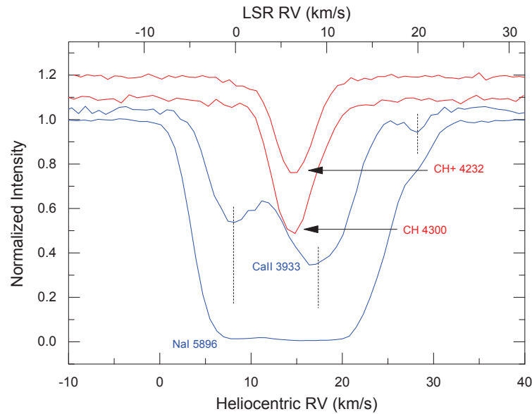
Fig. 4. Doppler structure of some interstellar lines, seen in HARPS-N (November 2013) spectrum of AE Aur. Atomic features are in blue, molecular ones in red. Different lines are slightly vertically displaced to make them more distinguishable. Vertical lines mark the central radial velocities of the resolved Doppler components in the CaII 3933 Å profile.
