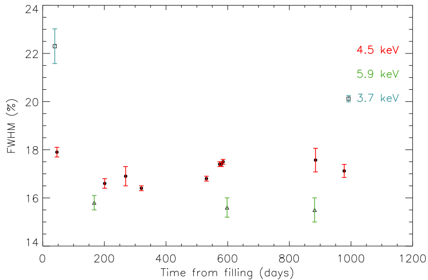
Figure 6. Energy resolution as a function of time since the GPD prototype mixture filling and sealing for three energies, 3.7, 4.5 keV and 5.9 keV. Only statistical uncertainties are shown. At least part of the point variation can be attributed to measurements not taken in the same conditions. Measurements were carried out on the same point of the detector with a pencil beam, and gain correction was not applied.
