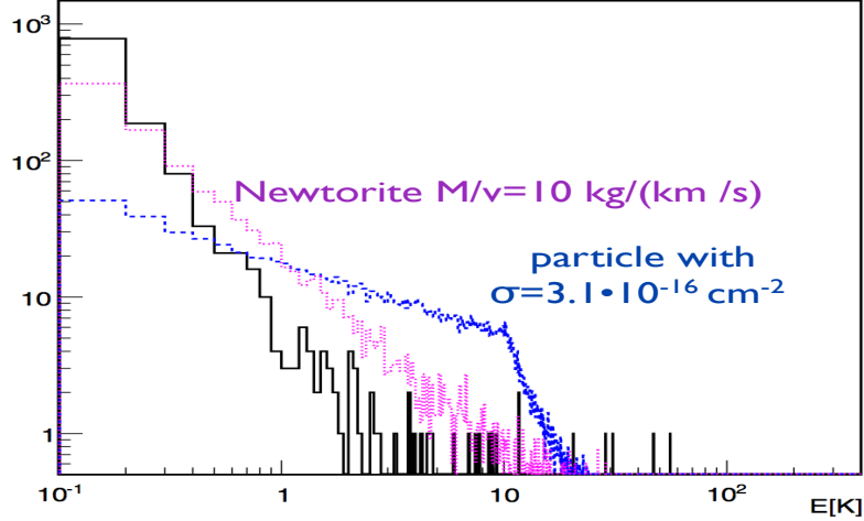
Figure 11: Nautilus 2005-2014 events energy distribution (continuous line) compared with the nuclearite Montecarlo with \beta\theta(M)=0.001 (dashed, blue online) and with the newtorite Montecarlo for M/v=10 kg s/km (dots, magenta online). For different values of M/v , eq.(11) shows that the mode energy scales with (M/v)^2 Montecarlo events are normalized in order to have the same number of events as the real data.
