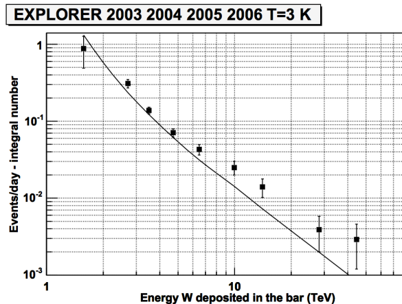
Figure 2: Integral distribution of extensive air showers in Explorer. The line shows the prediction based on the thermo acoustic model [32]. One event, the largest ever recorded, with an energy of 360 TeV. ( 670 K in kelvin units), sits at the far right outside this plot.
