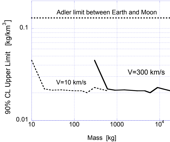
Figure 16: Newtorites density upper limits for v=10 and v=300 km/s vs the newtorite mass. The limits are obtained from the Nautilus 2011 data set. As the mass increases the limit reaches a plateau
