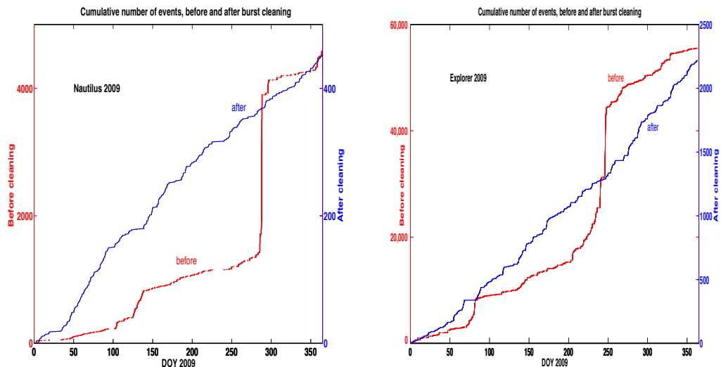
Figure 4: Cumulative time distribution of the Explorer and Nautilus events during year 2009. One can clearly see that there are periods with a rate of events orders of magnitude larger than in the quiet periods of operation. For each detector, we show the distribution before (red online) and after (blue online) the cuts operated to remove the noisy periods. The selections reduces the number of events by a factor between 10 and 20.
