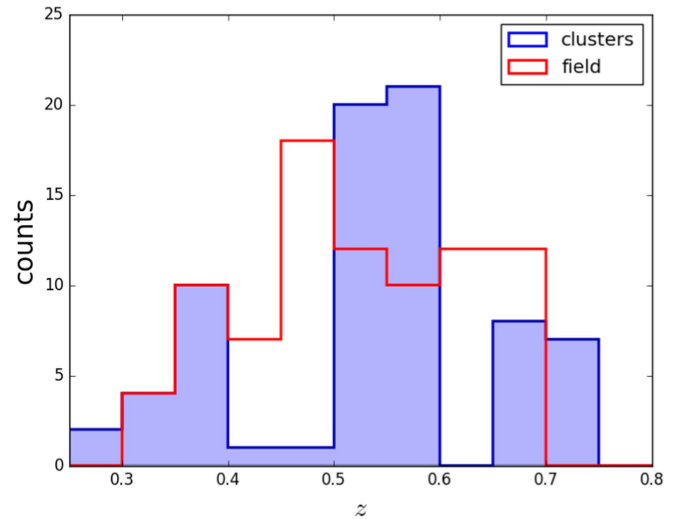
Figure 1. Redshift distribution for cluster (blue) and field (red) galaxies in our sample.
