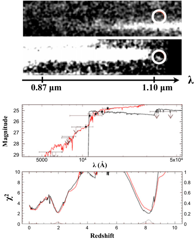
Figure 7. GLASS G102 spectra (top panels), photometry (central panel), and photometric redshift estimate \chi^2 curve (bottom panel) for the candidate Ly \alpha emitter at z = 8.1 , MACS2129_00899. The photometry includes CH1 and CH2 IRAC 1\sigma upper limits from SURFS-UP (Bradač et al. 2014) obtained following Huang et al. (2015). The black \chi^2 curve in the bottom panel includes F160W, whereas the red curve does not (F160W has potential contamination and therefore uncertain photometry). In both cases there are valid photometric redshifts around z \sim 8 (black spectral energy distribution overlotted on the photometry in the center panel) and z \sim 2 (red spectral energy distribution overlotted on the photometry in the center panel) with marginal statistical difference. The z \sim 2 solution overestimates the 1\sigma IRAC constraints. If the line were [O III] \lambda 3727 at z = 1.97 , we would expect to see [O III] at roughly 14870 \text{ \AA} . We do not detect any [O III] emission in the GLASS G141 spectra, consistent with the z \sim 8 solution.
