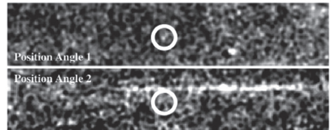
Figure 8. GLASS G141 spectra of the two potential line emitters at z \sim 10 from the Silver_EL sample. The white circles mark the detected line emission. The objects were selected as Lyman break dropouts. However, highly likely low-redshift solutions in the EA zY p(z) suggest that the lines could also be [O II] at z \sim 2.6 . Given the location of the lines at 1.32 and 1.37 \mu\text{m} , the G141 spectrum does not cover [O III], and the resolution does not allow us to resolve the potential [O II] doublet or detect the asymmetry of Ly \alpha . With the current data we therefore cannot rule out the high-redshift scenario.
