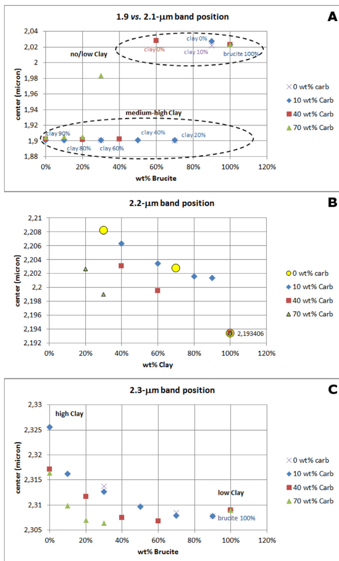
Fig. 7. A center of the 2.1 \mu m feature of brucite; this band rapidly disappears, while the clay 1.9 \mu m feature appears, as the clay content increases. B: center of the 2.2 \mu m feature of clay. C: center of the 2.3 \mu m feature of brucite. This band disappears while the clay 2.35 \mu m feature appears as the clay content increases.
