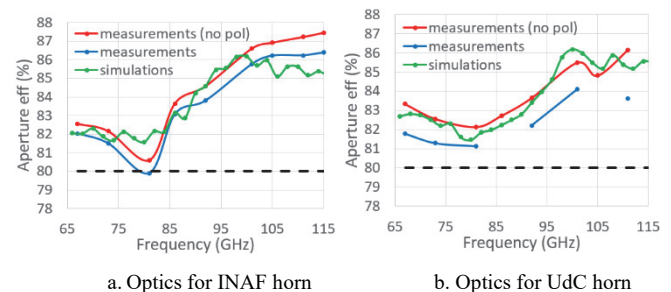
Fig. 3. Preliminary results of aperture efficiency calculations from measurements with prototype components, compared with simulations. Data labeled measurement (no pol) considers polarization efficiency = 100%
