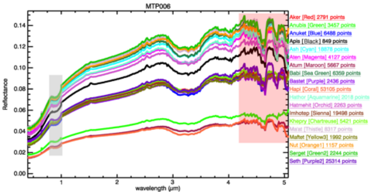
Figure 16: Average VIS-IR reflectance spectra of the nineteen morphological regions. For each region are indicated the number of points, corresponding to 0.5 \times 0.5^\circ bins on cylindrical map projection, used to compute the average spectra. In gray the visible spectral range affected by low signal to noise conditions. In red the infrared range affected by thermal emission removal method, calibration residuals and detector’s non-linearity response.
