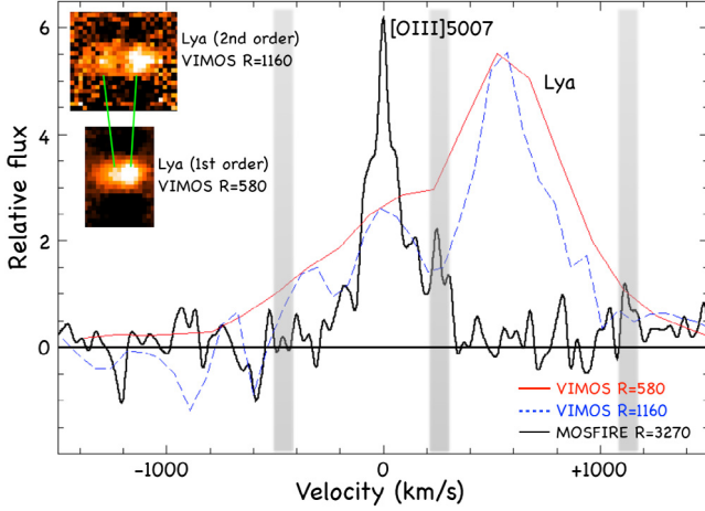
Fig. 9. Velocity profiles of [O III] \lambda 5007 and Ly \alpha lines relative to systemic. The [O III] \lambda 5007 line is shown in black, the Ly \alpha first order in red, and the Ly \alpha second order with the dashed blue line. The positions and widths of the sky lines are indicated by gray stripes.
