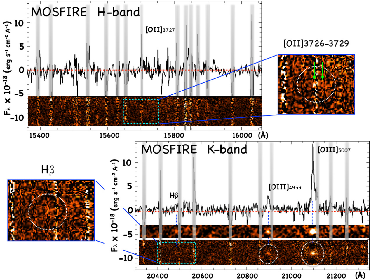
Fig. 4. Two- and one-dimensional near-infrared spectra of Ion2 in the MOSFIRE H - and K -band. Two insets show the regions where H \beta and the [O II] \lambda 3727 doublet are expected from the redshift. The gray stripes in the one-dimensional spectra indicate the position of the sky lines.
