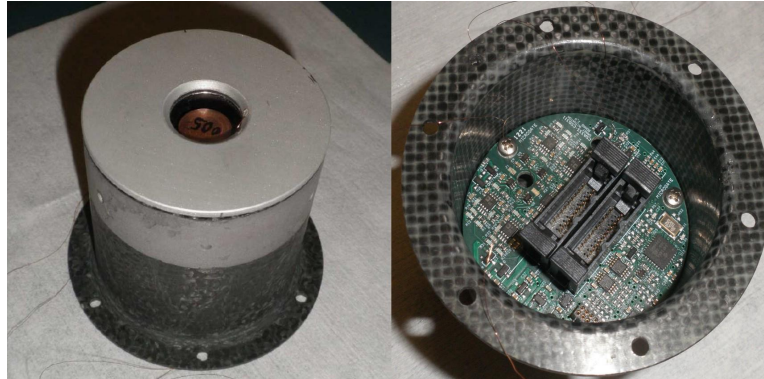
Figure 6. Smart actuator board
